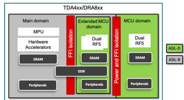
Figure 1. Jacinto 7 platform safety architecture
