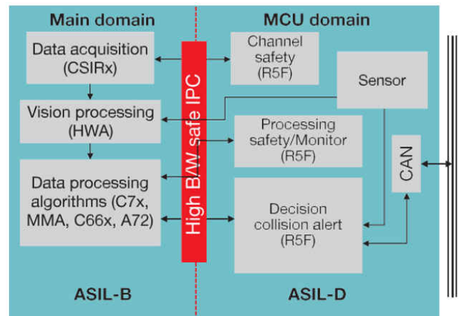
Figure 2. Typical Vision Processing
