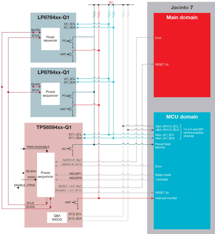
Figure 3. TPS6594-Q1 + LP8764-Q1 + LP8764-Q1 Communication as “Virtual” PMIC
