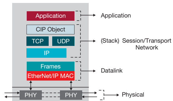
Figure 5. EtherNet/IP node.
