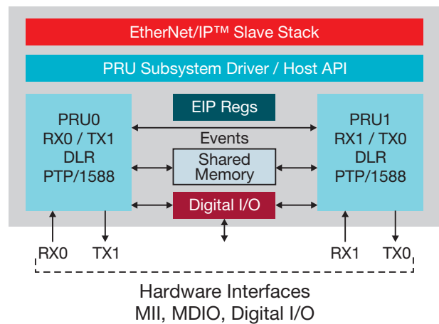
Figure 10. Firmware architecture.
