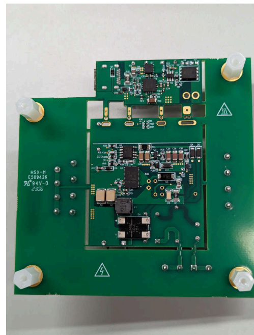
LMG3622EVM-082 (底视图)
