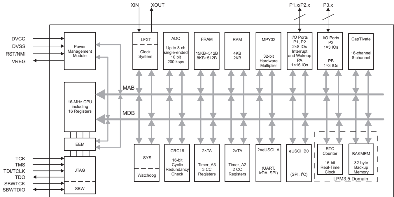
图 2. Block Diagram of MSP430FR2633
