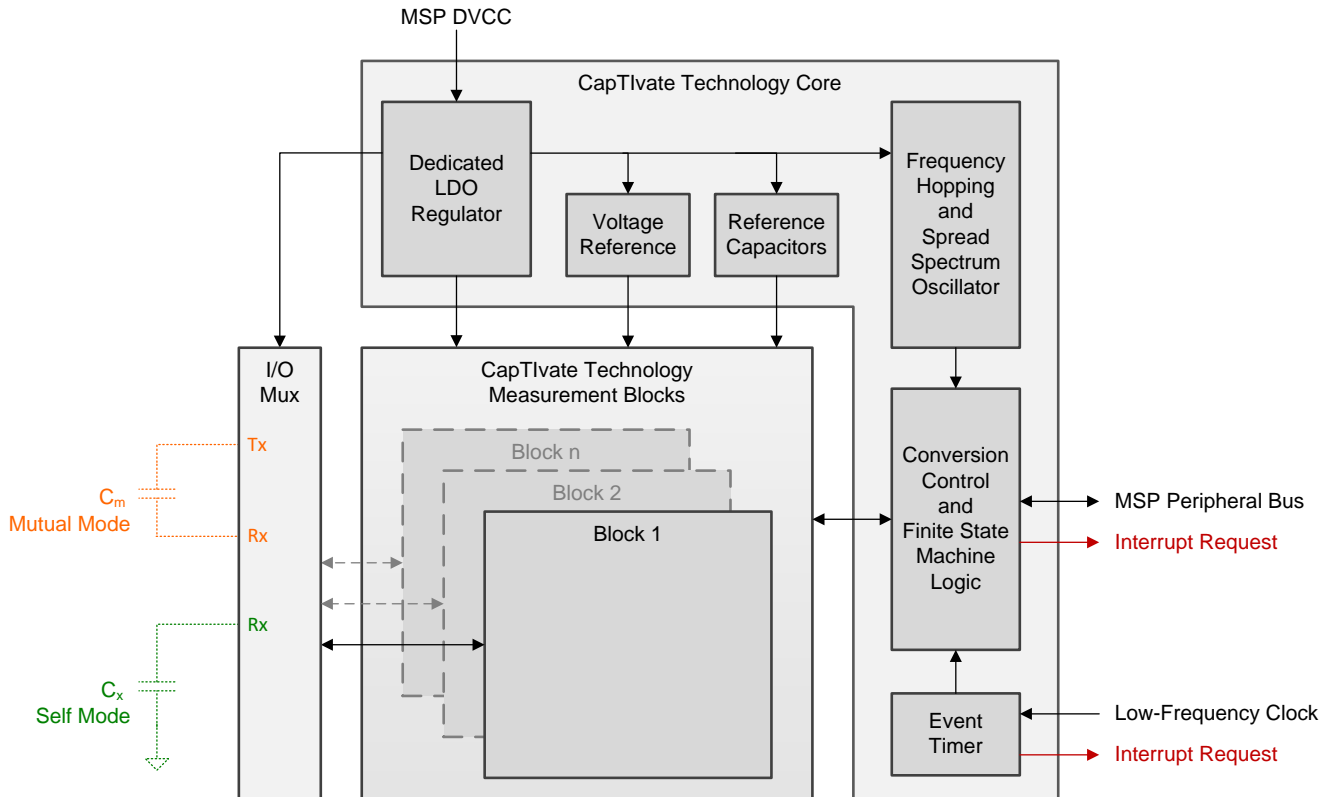
图 3. CapTlvate Technology Block Diagram
