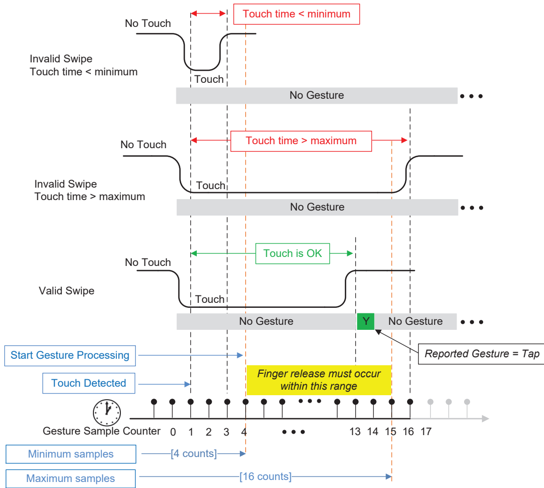
图 7. Tap Gesture Detection
