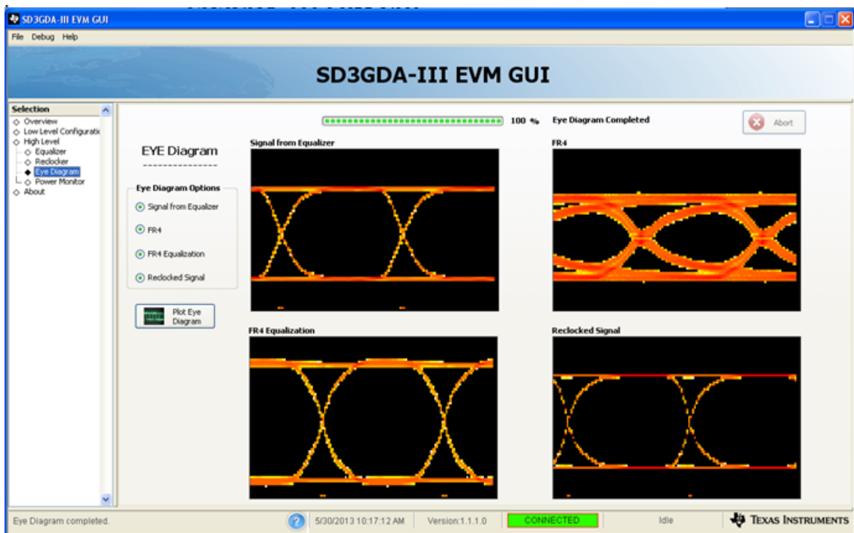
Figure1. Eye Diagrams after the Equalizer and Reclocker at the end of different media
