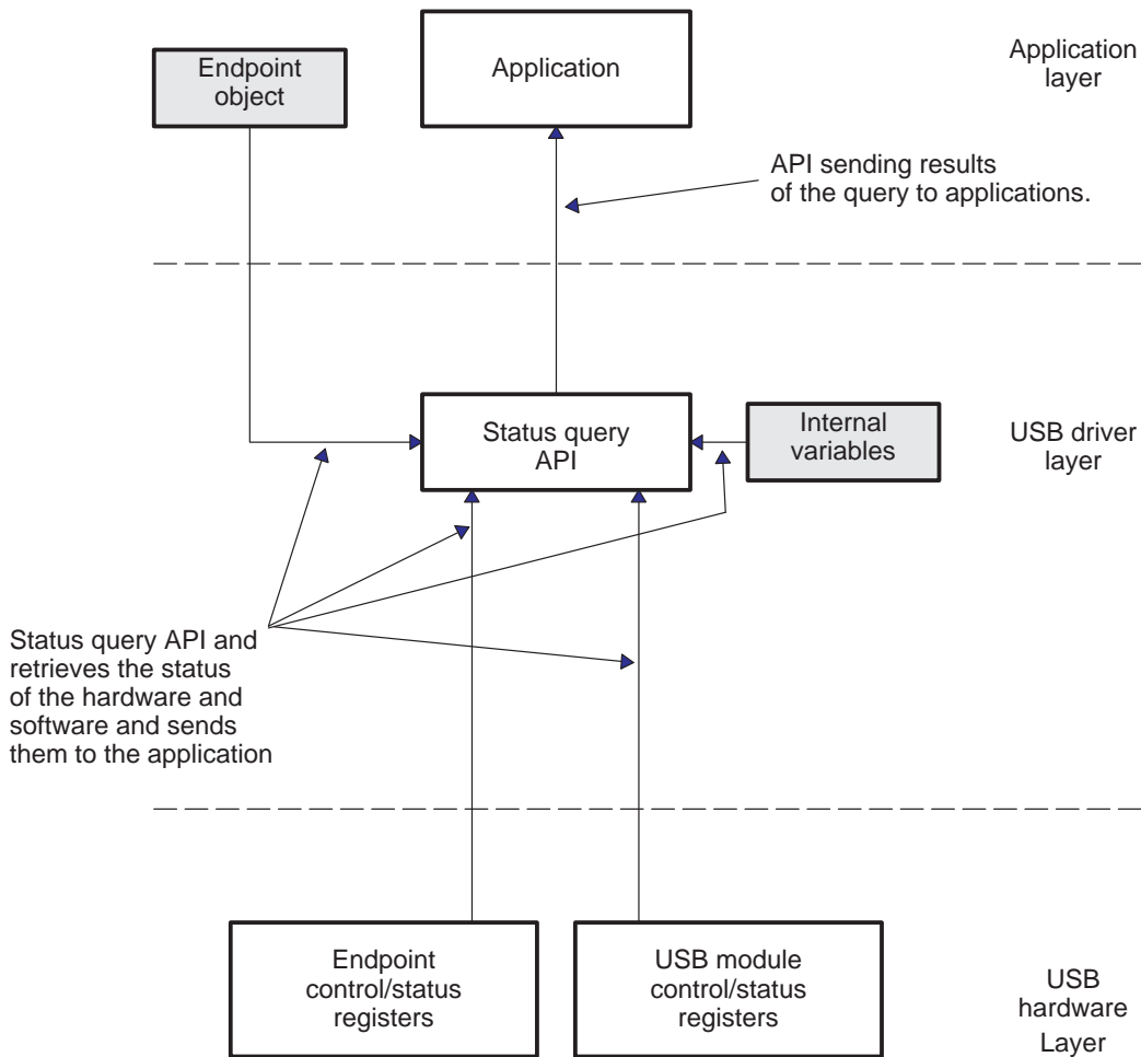
Figure 1–6. Status Query
