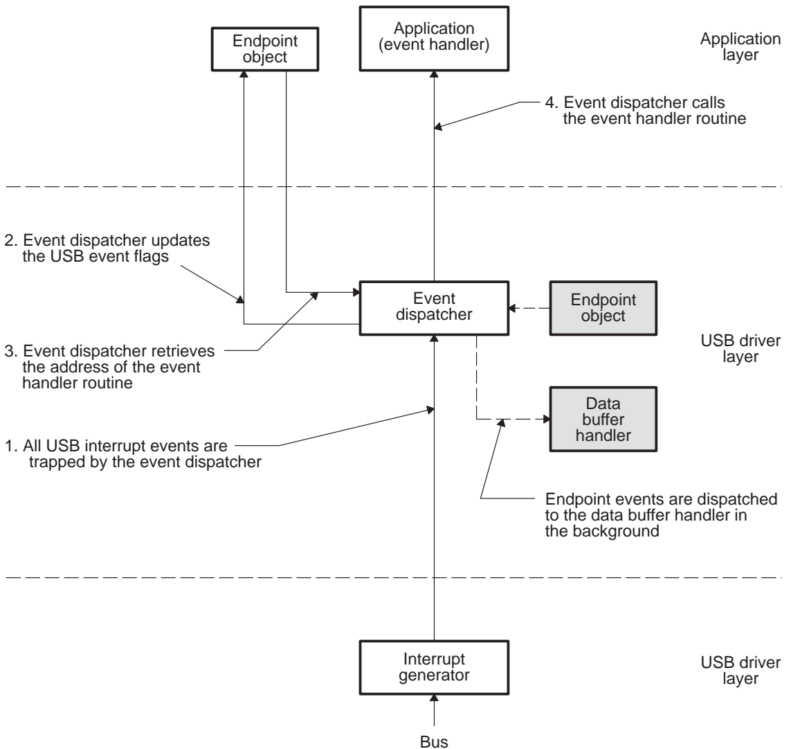
Figure 1–8. Event Dispatcher
