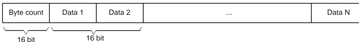
Figure 1–1. Endpoint Data Buffer Format
