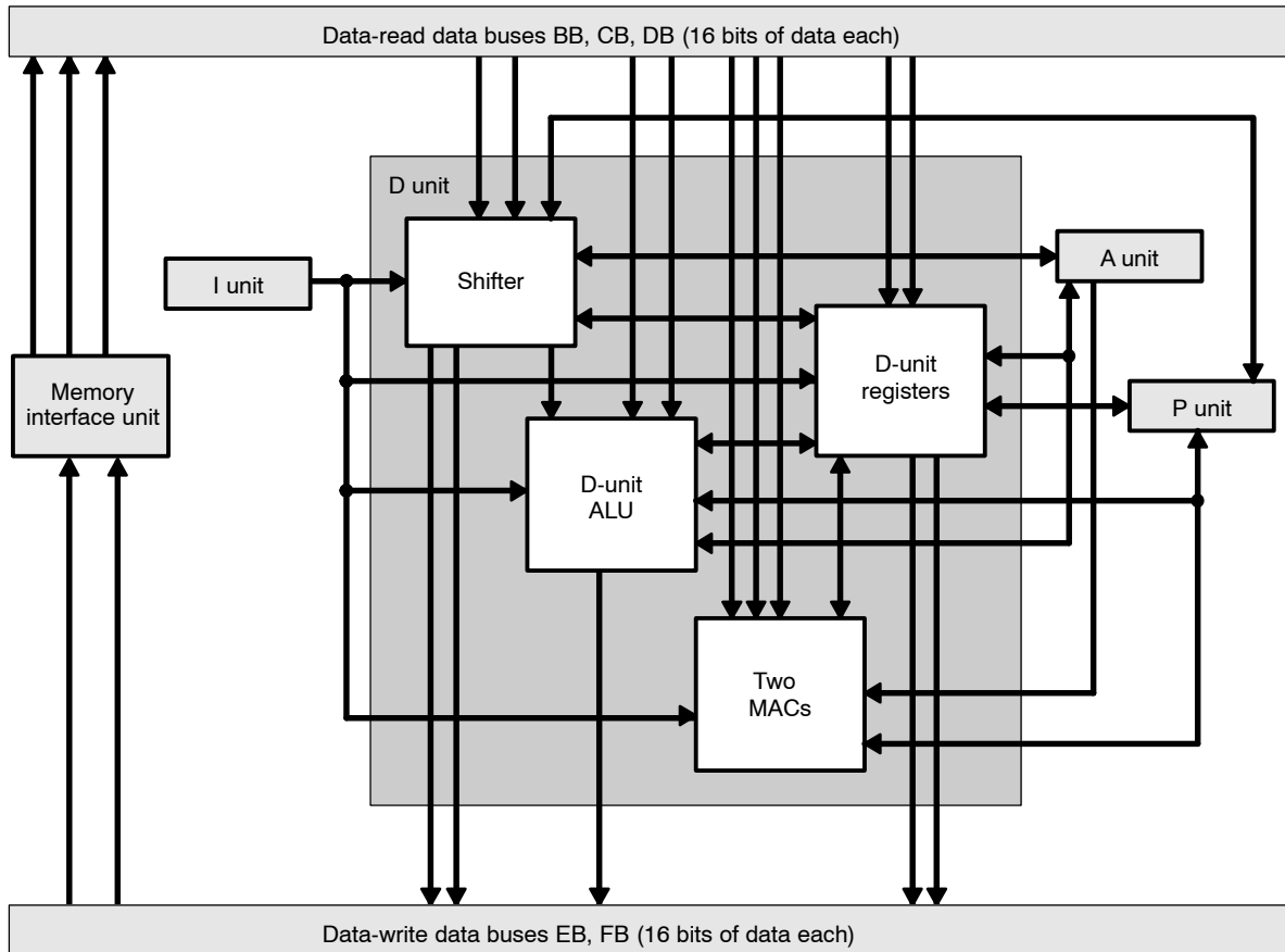
Figure 1–5. Data Computation Unit (D Unit) Diagram
