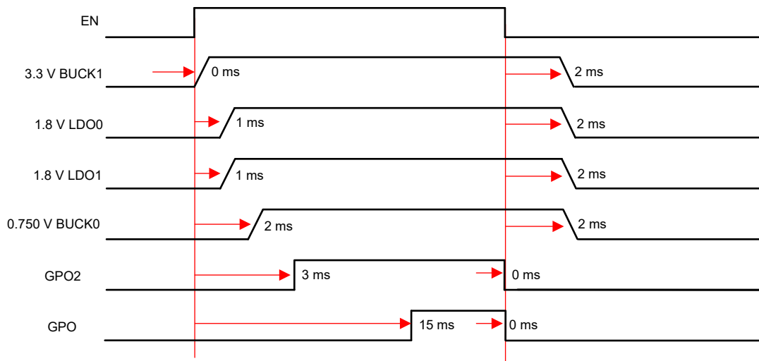
Figure 3-1. LP873364 Power-up and Power Down Sequence
