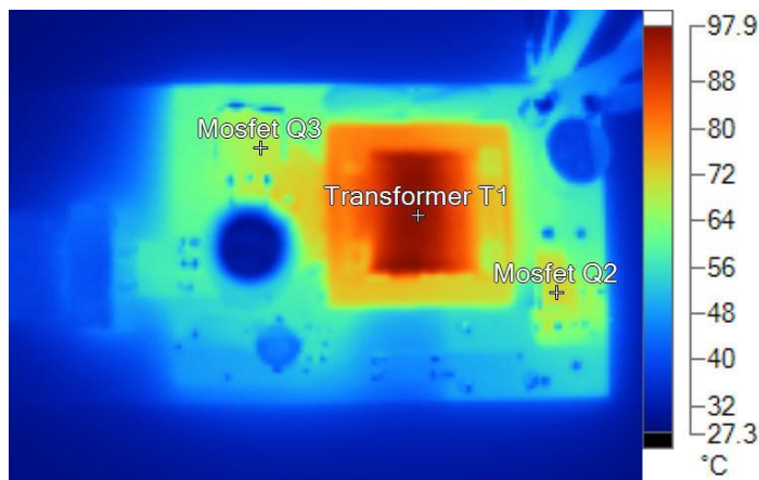
IR20131213_0408 Vin=265VC I=4.2A.is2
