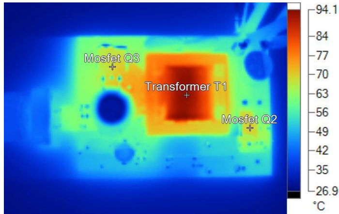
IR20131213_0407 Vin=195VAC I=4.2A.is2
