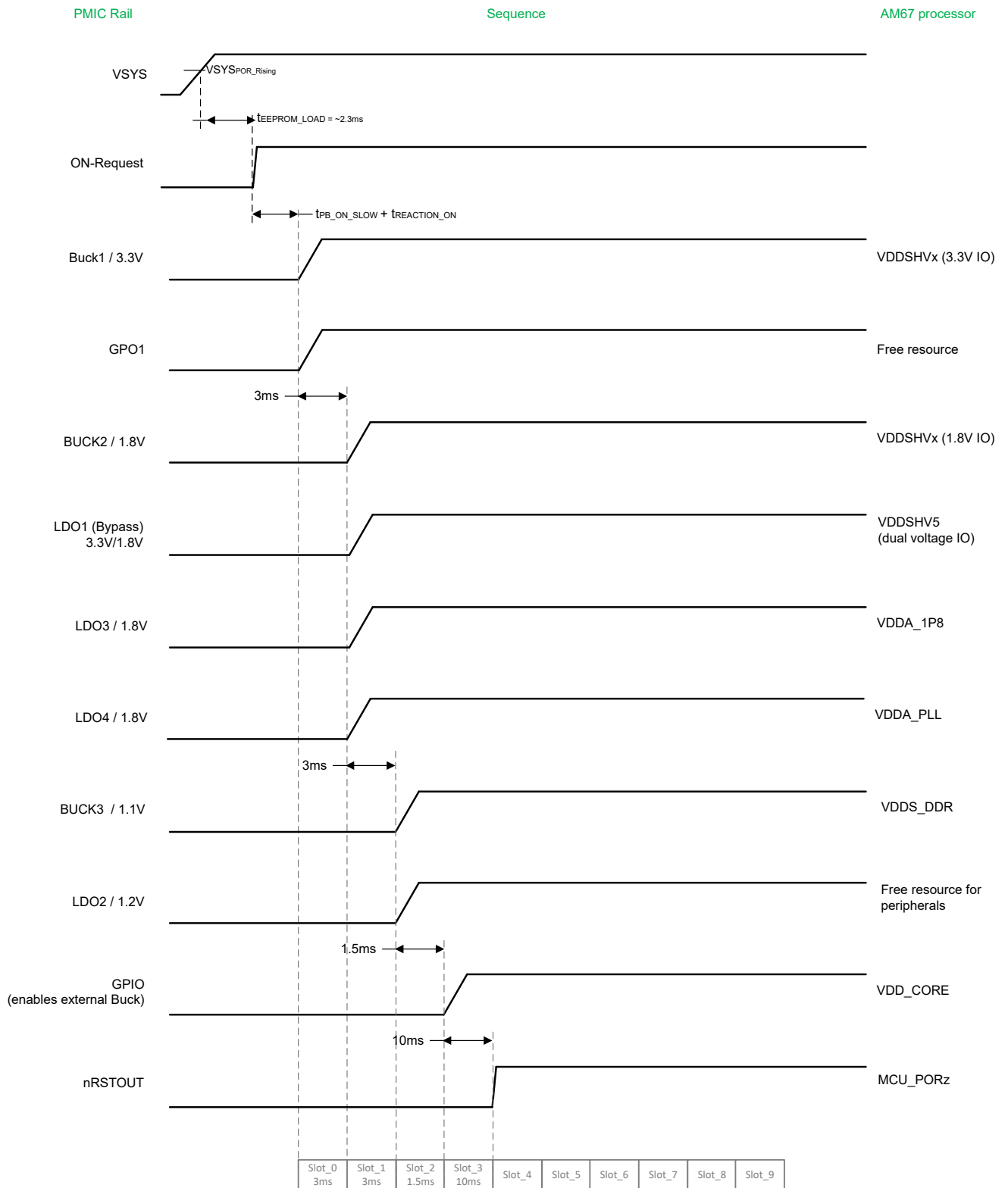
Figure 2-3. TPS6521910 Power-Up Sequence
