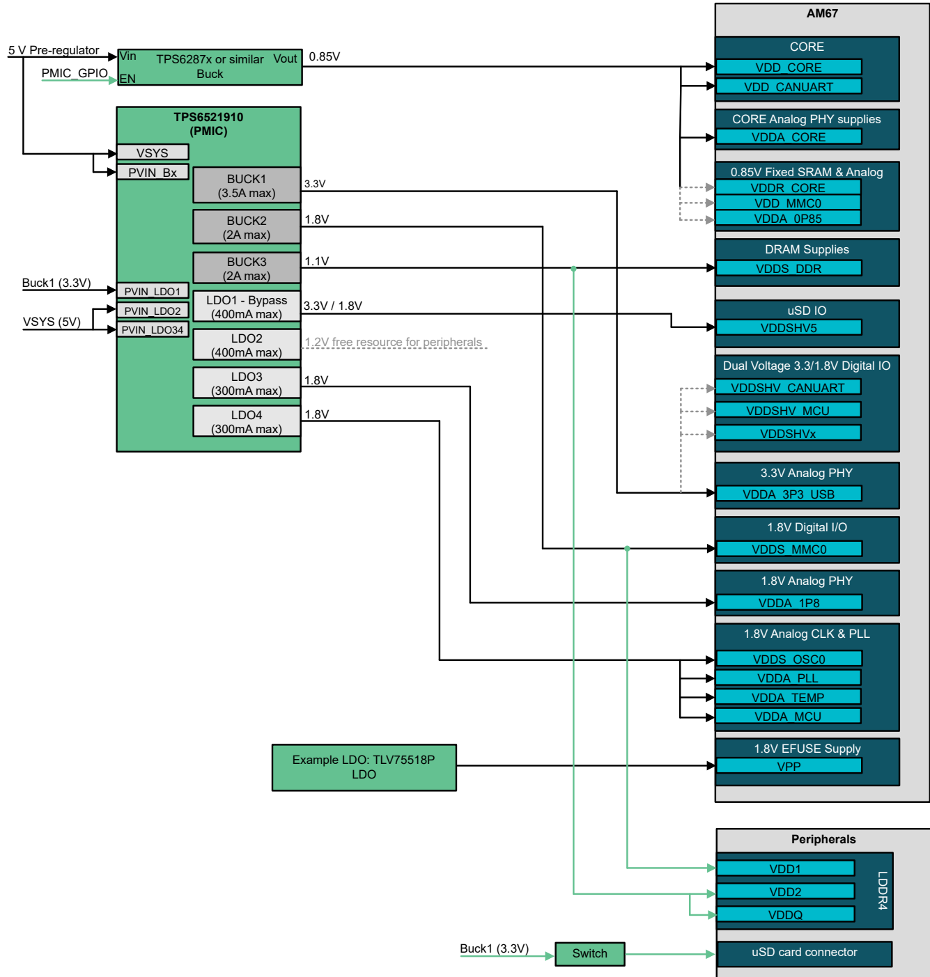
Figure 2-1. TPS6521910 Example Power Block Diagram
