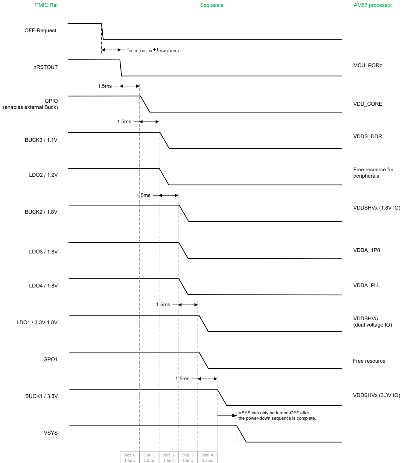
Figure 2-4. TPS6521910 Power-Down Sequence
