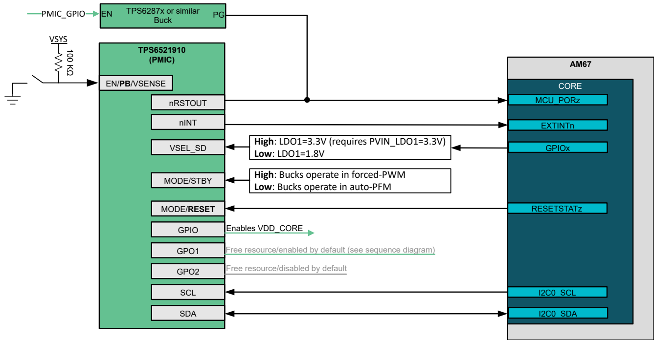
Figure 2-2. TPS6521910 Digital connections to AM67
