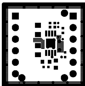
Figure 8. SMP-TPS7A1650-MVK Board Solder Mask – Top Side
