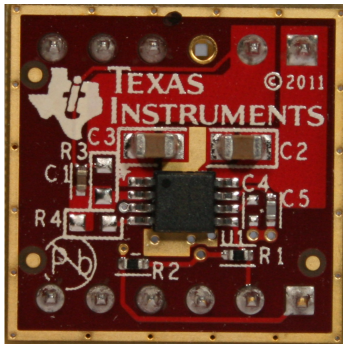
Figure 1. SMP-TPS7A1650-MVK MAVRK Submodule
