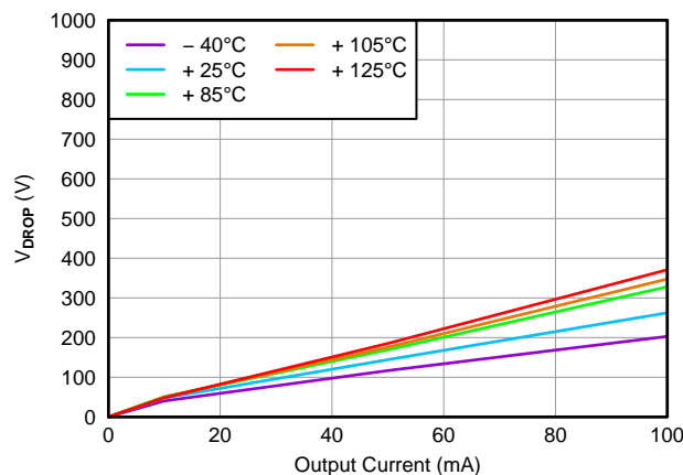
Figure 3. TPS7A1650 Dropout Voltage Versus Output Current
