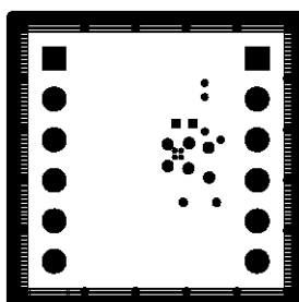
Figure 9. SMP-TPS7A1650-MVK Board Solder Mask – Bottom Side
