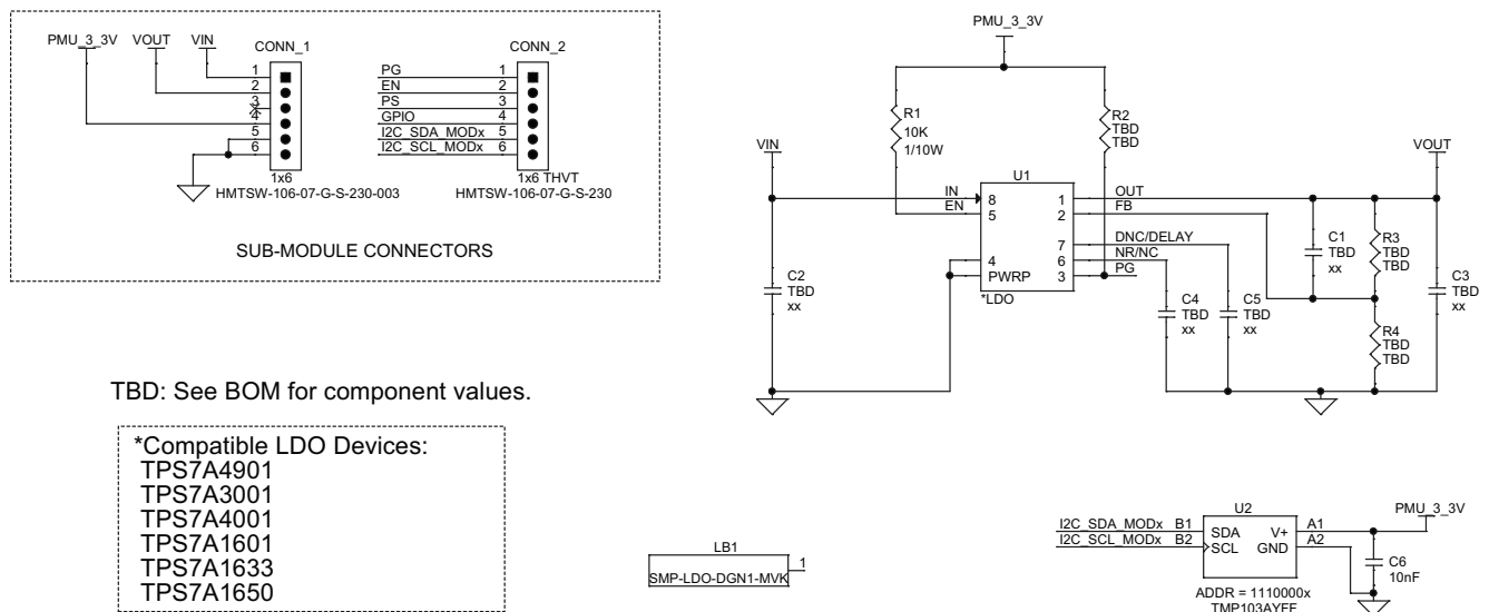
Figure 14. SMP-TPS7A1650-MVK Schematic
