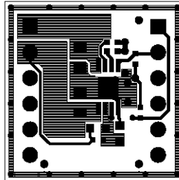
Figure 4. SMP-TPS7A1650-MVK Board Layer 1 – Top Side
