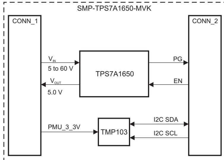
Figure 2. SMP-TPS7A1650-MVK Block Diagram
