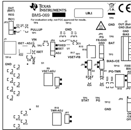
Figure 3-1. Top Overlay
