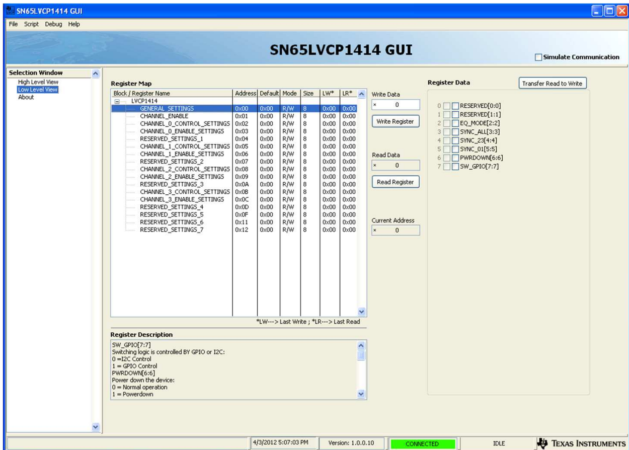
Figure 4. SN65LVCP1414 EVM GUI Low-Level Register Configuration Window
