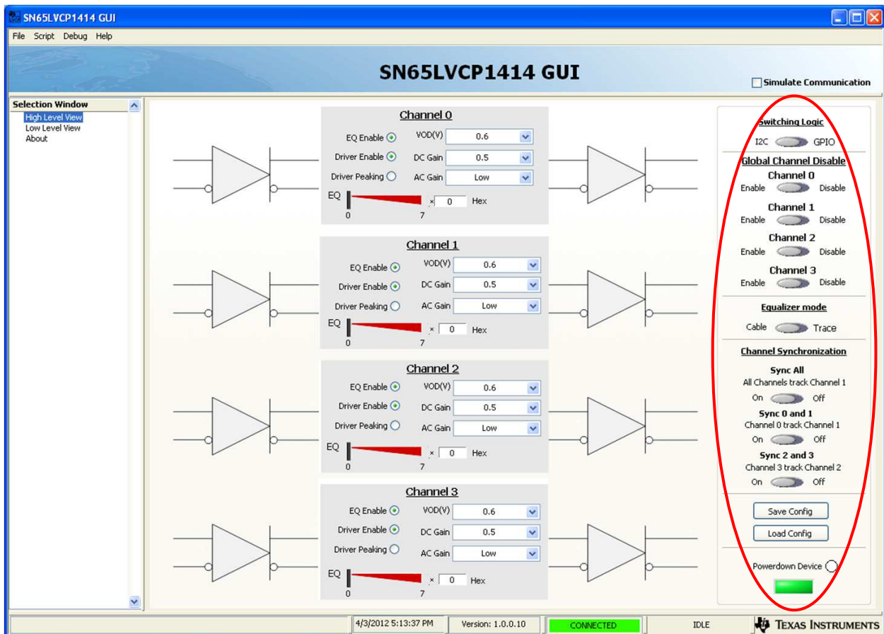
Figure 3. SN65LVCP1414 EVM GUI Global Settings
