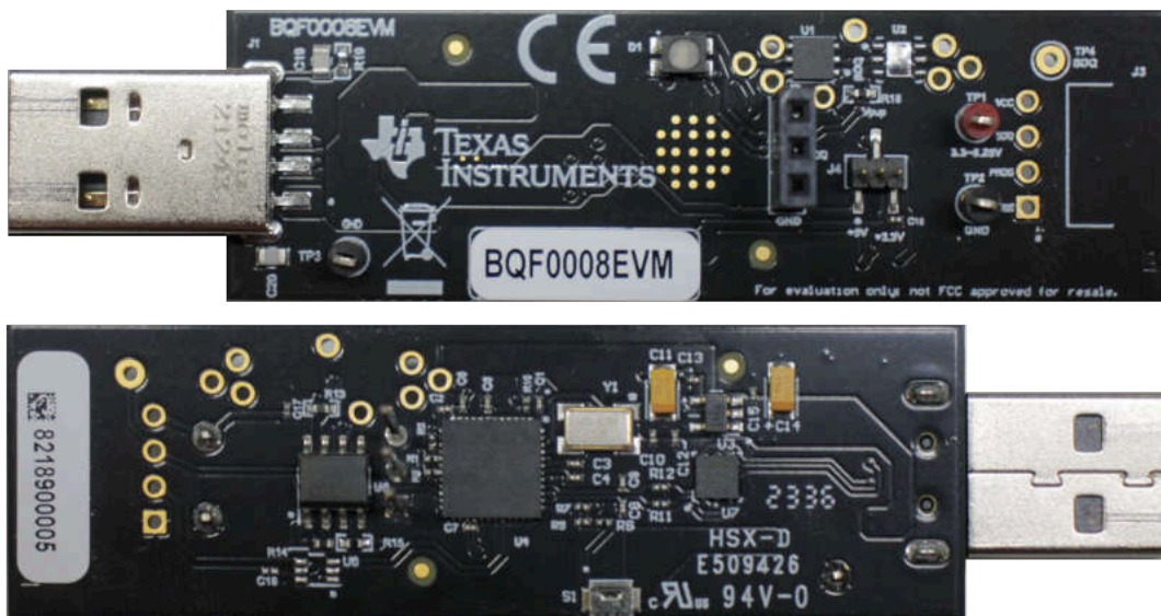
BQF0008EVM (顶视图和底视图)
