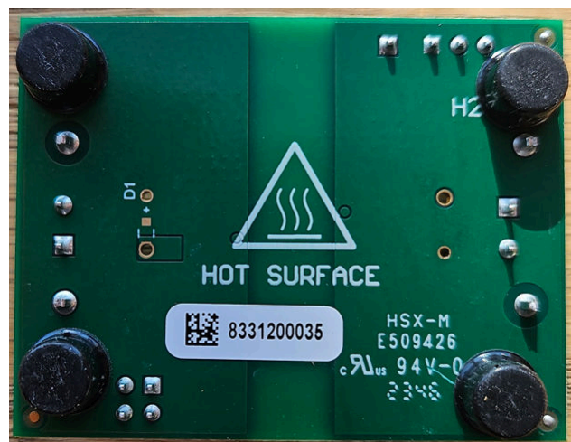
UCC33421EVM-092 (底视图)
