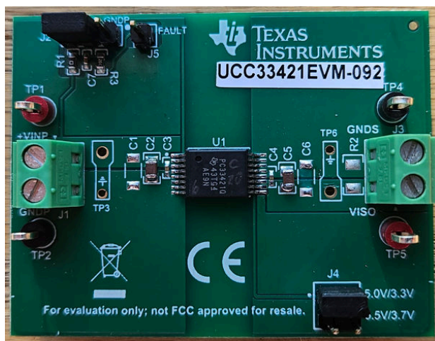
UCC33421EVM-092 (顶视图)
