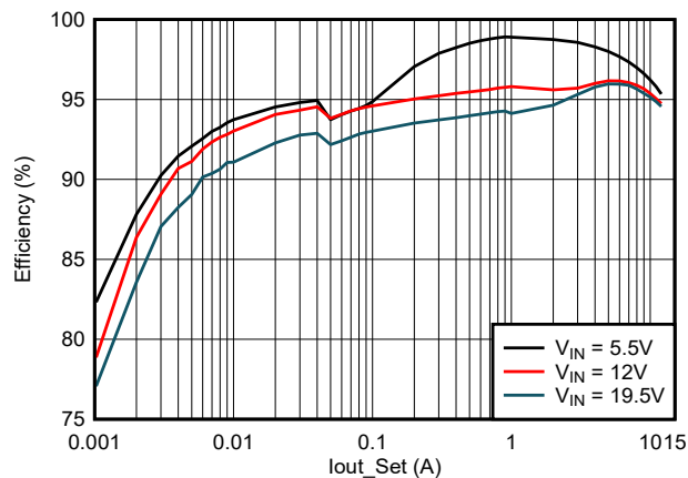
图 3-1. 效率, V_{EN} = 3.3V (Eco-mode), V_{OUT} = 5.15V , 560kHz
