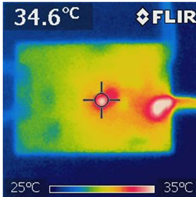
图 5-12. 热性能，强制 PWM ( V_{IN} = 12V , V_{OUT} = 3.3V , I_{OUT} = 1A , F_{sw} = 2.5MHz )
