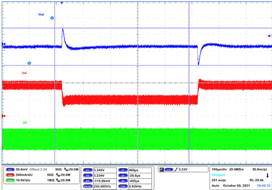
图 5-11. 负载瞬态，强制 PWM VSET ( V_{IN} = 12V , V_{OUT} = 3.3V , I_{OUT} = 0.5A - 1A , 压摆率 = 1A/\mu s )
