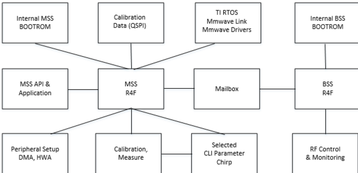
图 6. IWR1443 BOOST MSS/BSS Software Block Diagram
