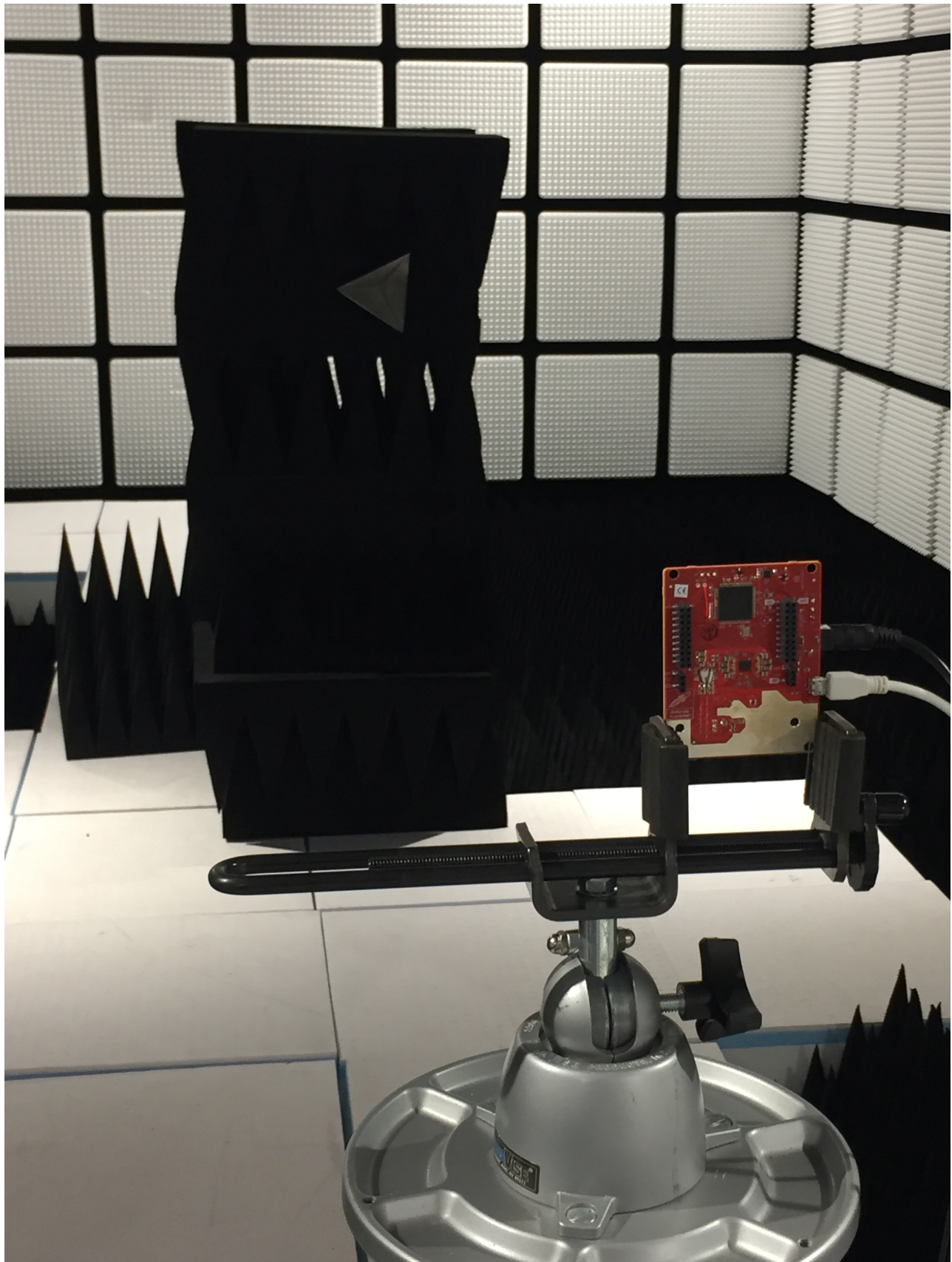
图 14. Range Measurement Setup
