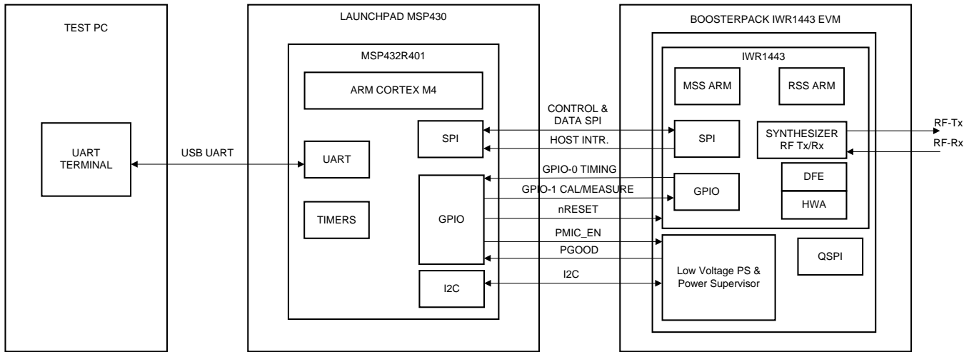
图 3. TIDEP-0091 mmWave Sensor IWR1443 BOOST and MSP432R401 EVM Diagram
