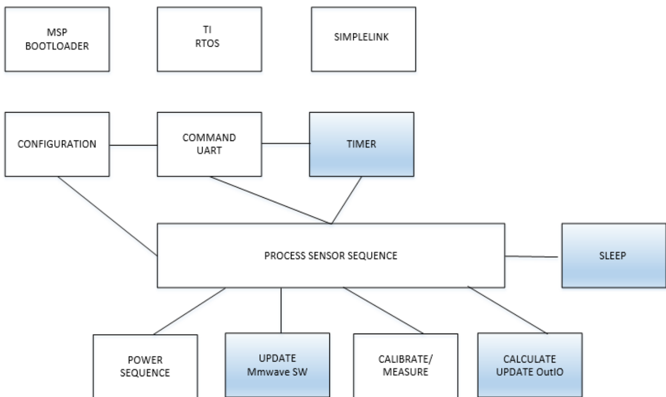
图 4. TIDEP-0091 MSP432 Host Processor Software Flow (Blue Boxes are Not Implemented)
