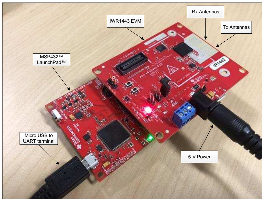
图 9. Level Sensing Demonstration Hardware
