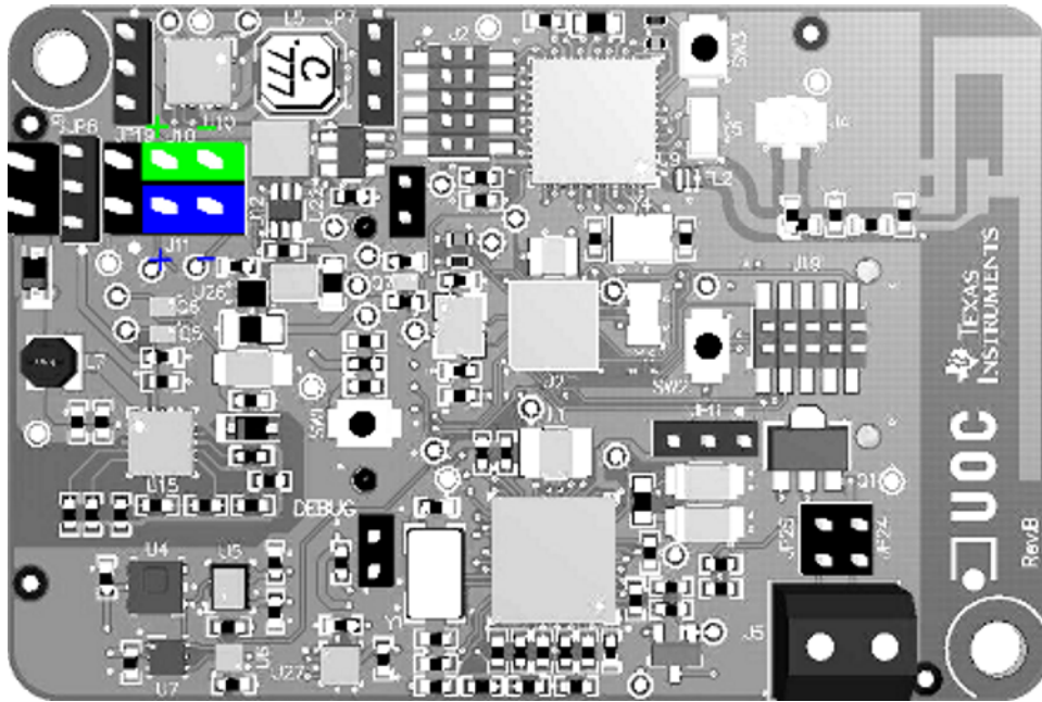
图 11. Primary Battery Input (Blue) and Secondary Rechargeable Battery Input (Green)
