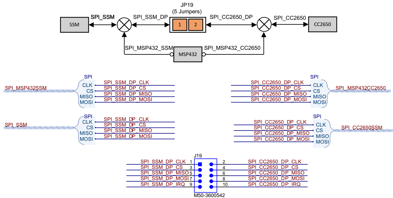
图 14. Settings to Connect SSM-SPI With CC2650 Directly or Through MSP432
