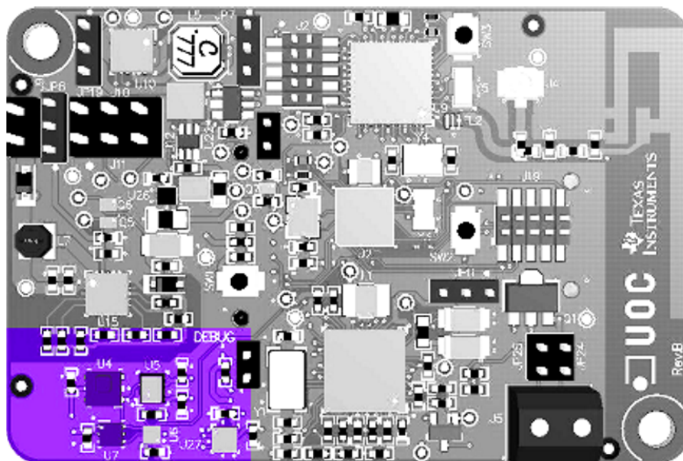
图 7. Onboard General Purpose Sensors Subsystem on I3Mote
