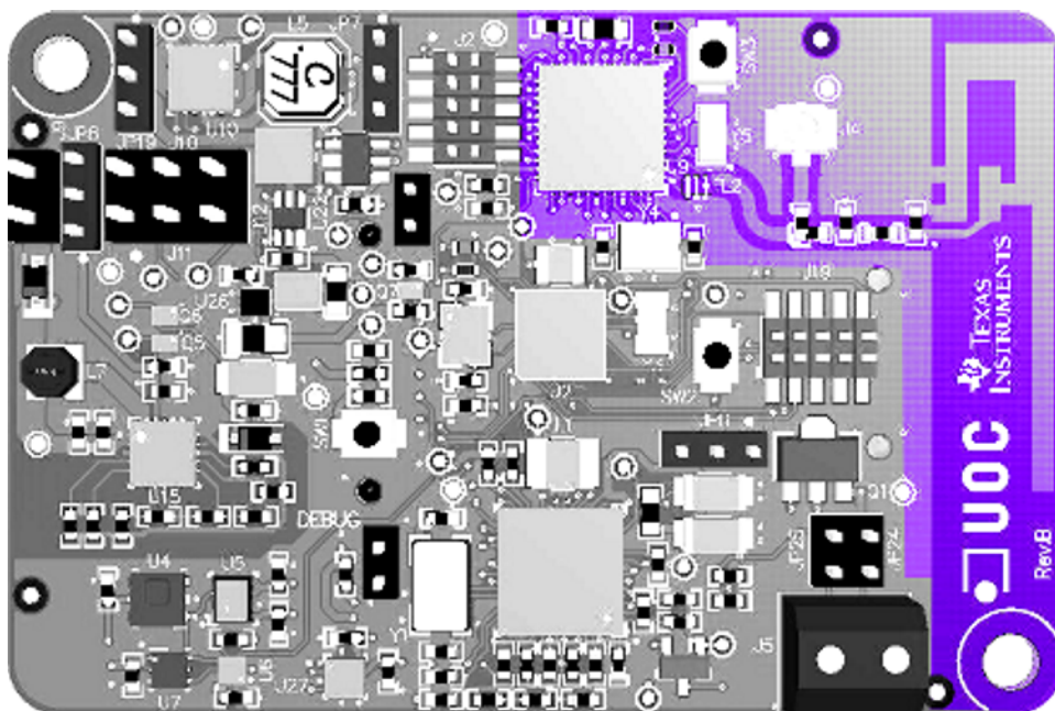
图 6. Wireless Communications Subsystem on I3Mote
