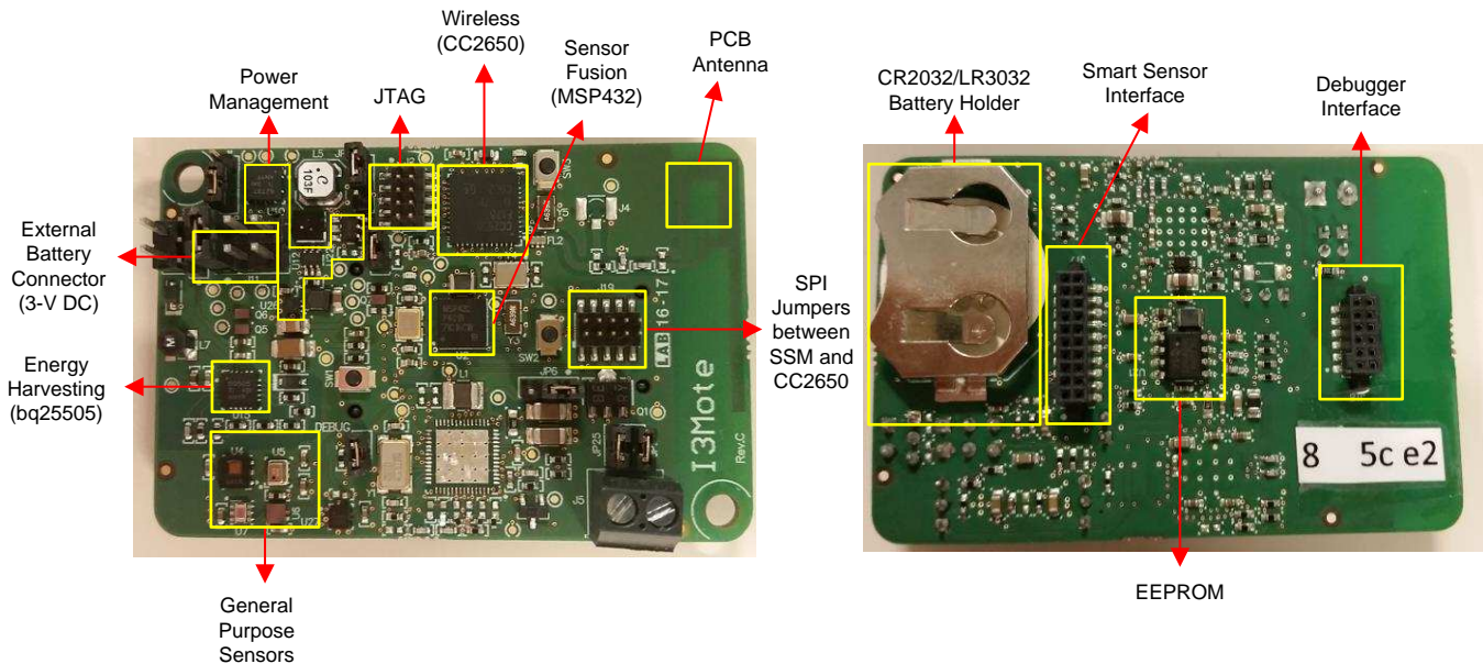
图 2. I3Mote Hardware Component Description
