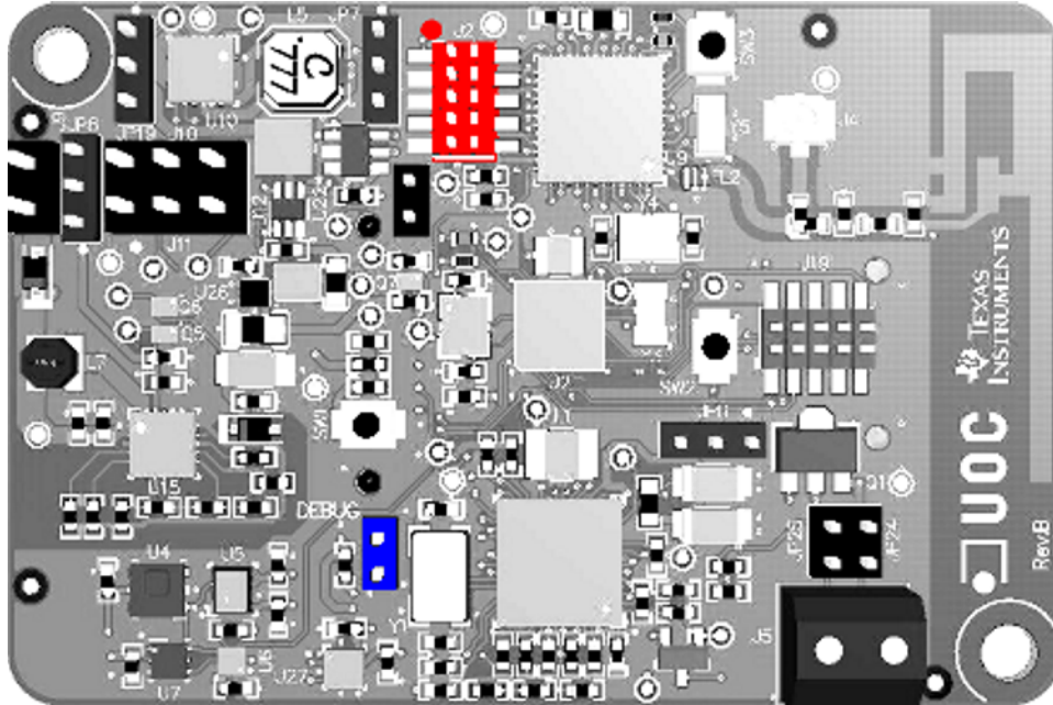
图 13. Daisy-Chained JTAG for MSP430™ and CC2650
