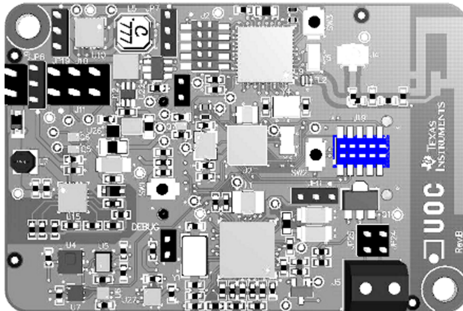
图 15. Jumper Settings for MSP432 Data Path J19: 1-2, 3-4, 5-6, 7-8, 9-10
