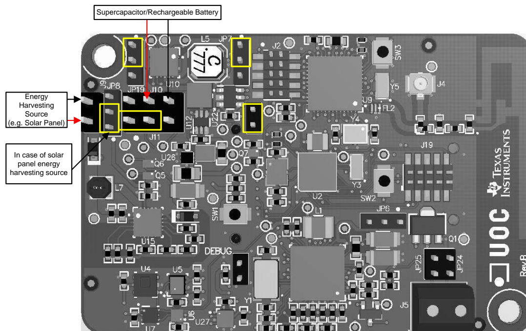
图 19. Jumper Configuration When Using Coin-Cell Battery (CR2032) and Energy Harvesting Source as Power Source
