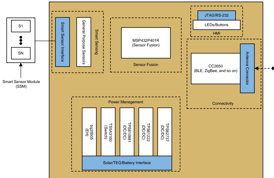
图 1. I3Mote Features
