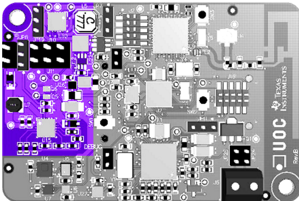
图 3. Power Management Subsystem of I3Mote
