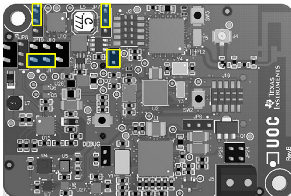
图 17. Jumper Configuration When Using Coin-Cell Battery as Power Source
