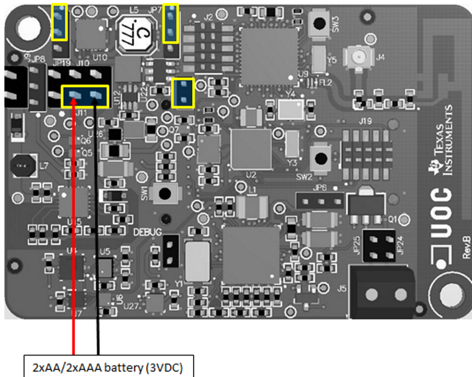
图 16. Jumper Configuration When Using 2xAA or 2xAAA Batteries as Power Source
