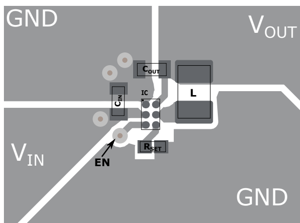
图 62. Recommended PCB Layout YBG Package
