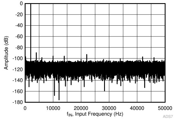
图 6-6. Typical FFT in Manual Mode
