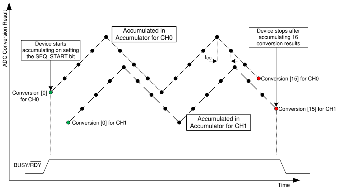
图 7-25. High-Precision Mode With Dual-Channel Configurations
