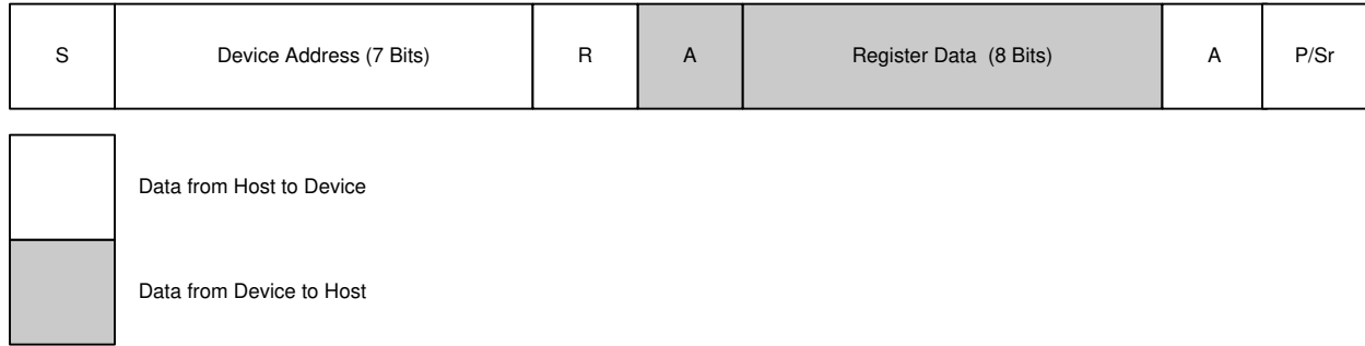
图 7-27. Reading Register Data
