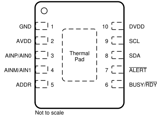
图 5-1. DQC Package, 10-Pin WSON (Top View)
