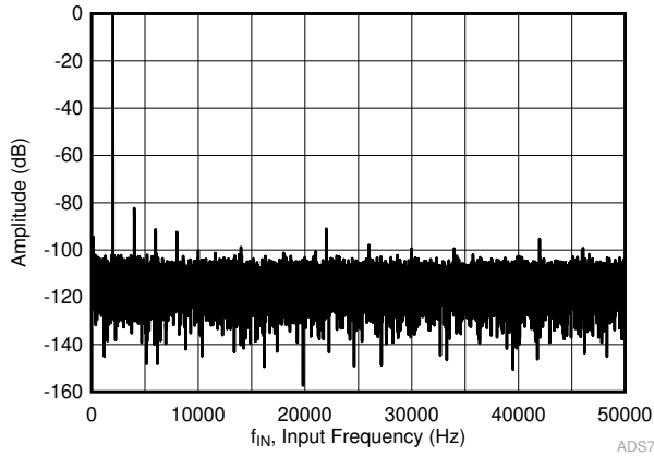
图 6-5. Typical FFT in Manual Mode
