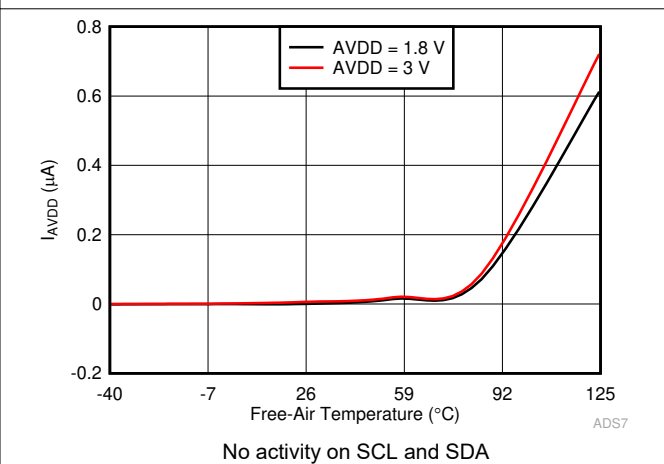
图 6-28. Static I_{AVDD} in Manual Mode vs Temperature
