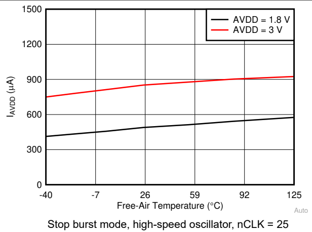
图 6-32. I_{AVDD} in Autonomous Modes vs Temperature
