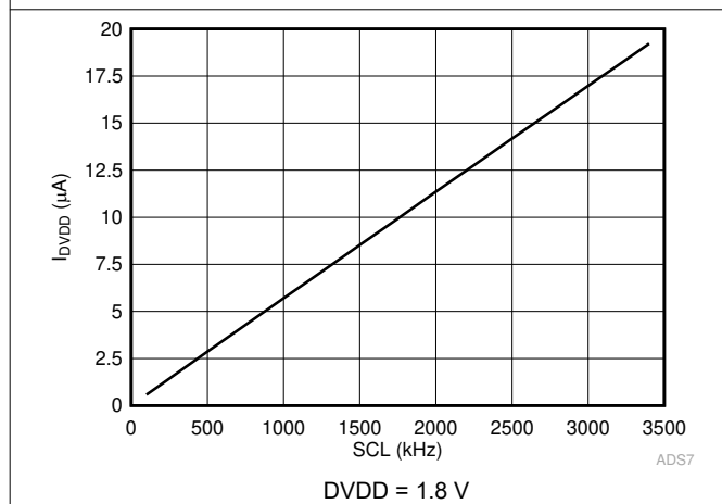
图 6-27. I_{DVDD} in Manual Mode vs SCL
