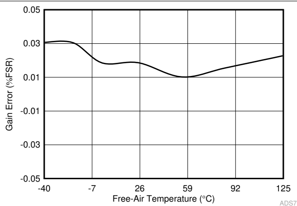
图 6-15. Gain Error in Manual Mode vs Free-Air Temperature
