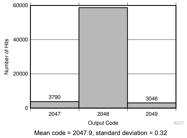
图 6-12. Typical DC Code Spread in Manual Mode
