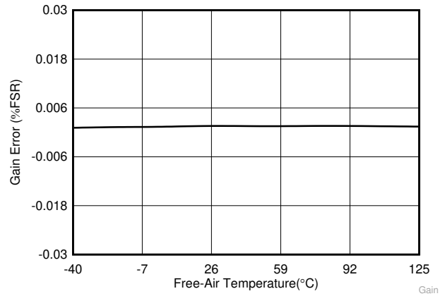
图 6-34. Gain Error in High-Precision Mode vs Temperature
