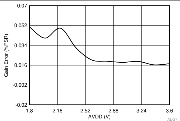
图 6-16. Gain Error in Manual Mode vs AVDD
