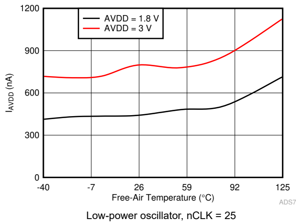
图 6-35. I_{AVDD} in High-Precision Mode vs Temperature Low-power oscillator, nCLK = 25
