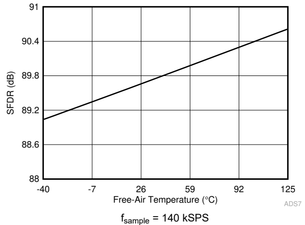
图 6-10. SFDR in Manual Mode vs Temperature
