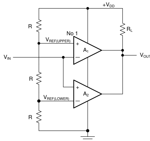
图 8-1. Analog Window Comparator
