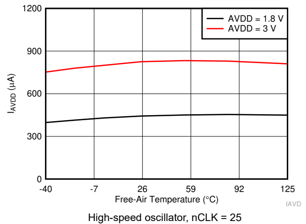
图 6-36. I_{AVDD} in High-Precision Mode vs Temperature High-speed oscillator, nCLK = 25
