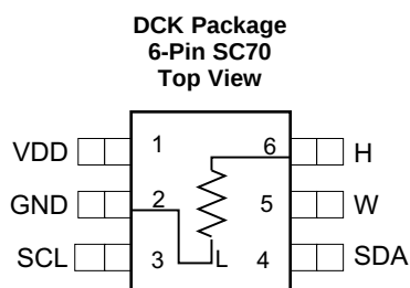
Pin Functions
