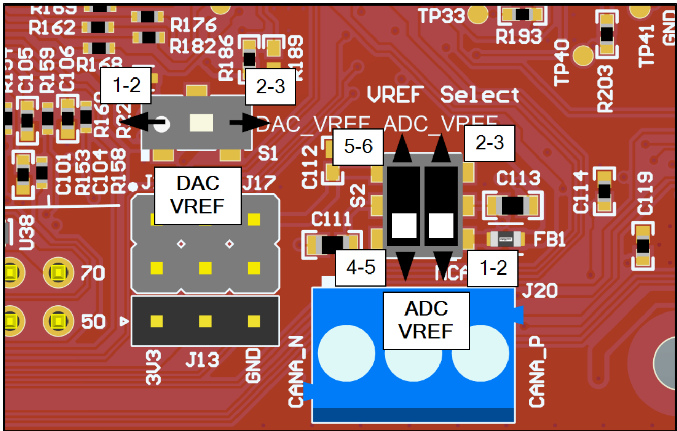
Figure 2-31. LP-AM261 ADC/DAC VREF Switches
