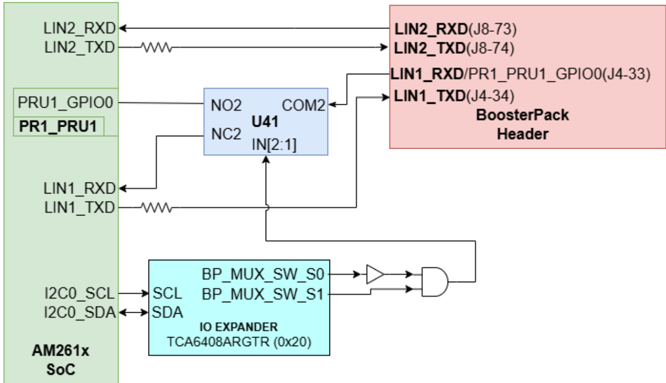
Figure 2-27. LIN Instances to BoosterPack Header
