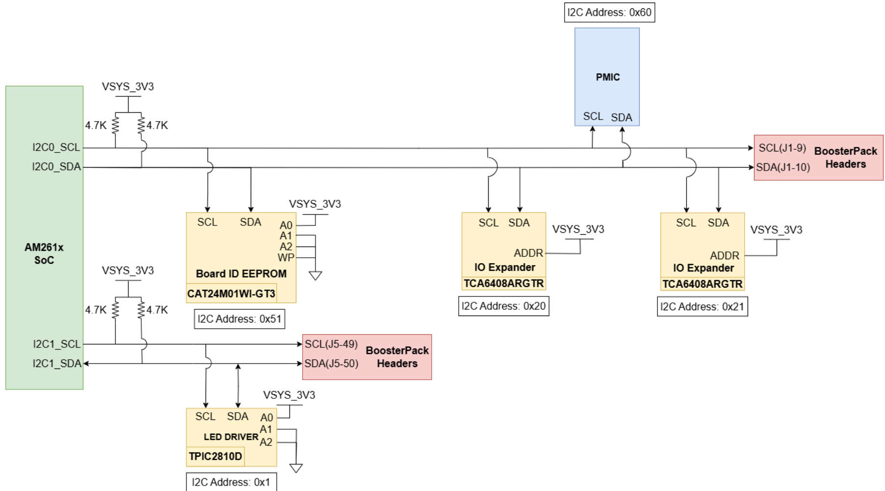
Figure 2-18. LP-AM261 I2C Interface
