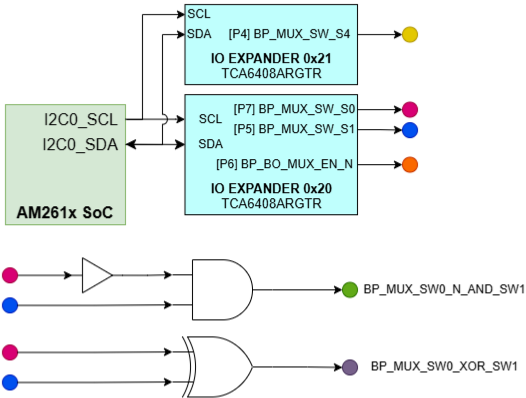
Figure 2-28. BoosterPack Mode Mux Select Logic
