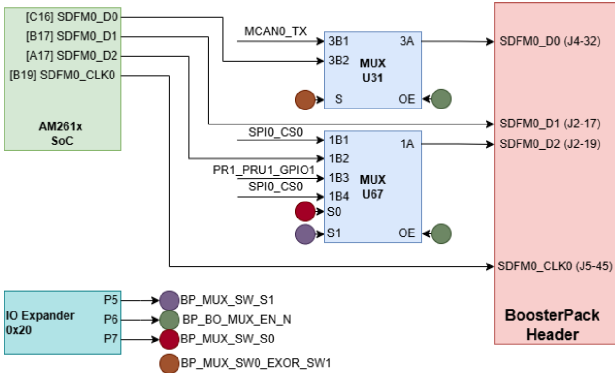
Figure 2-23. SDFM0
