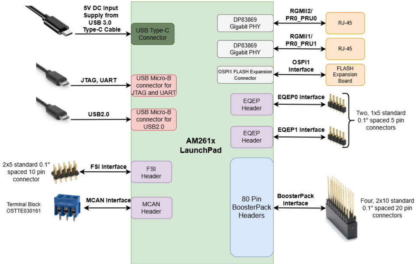
Figure 1-1. System Architecture
