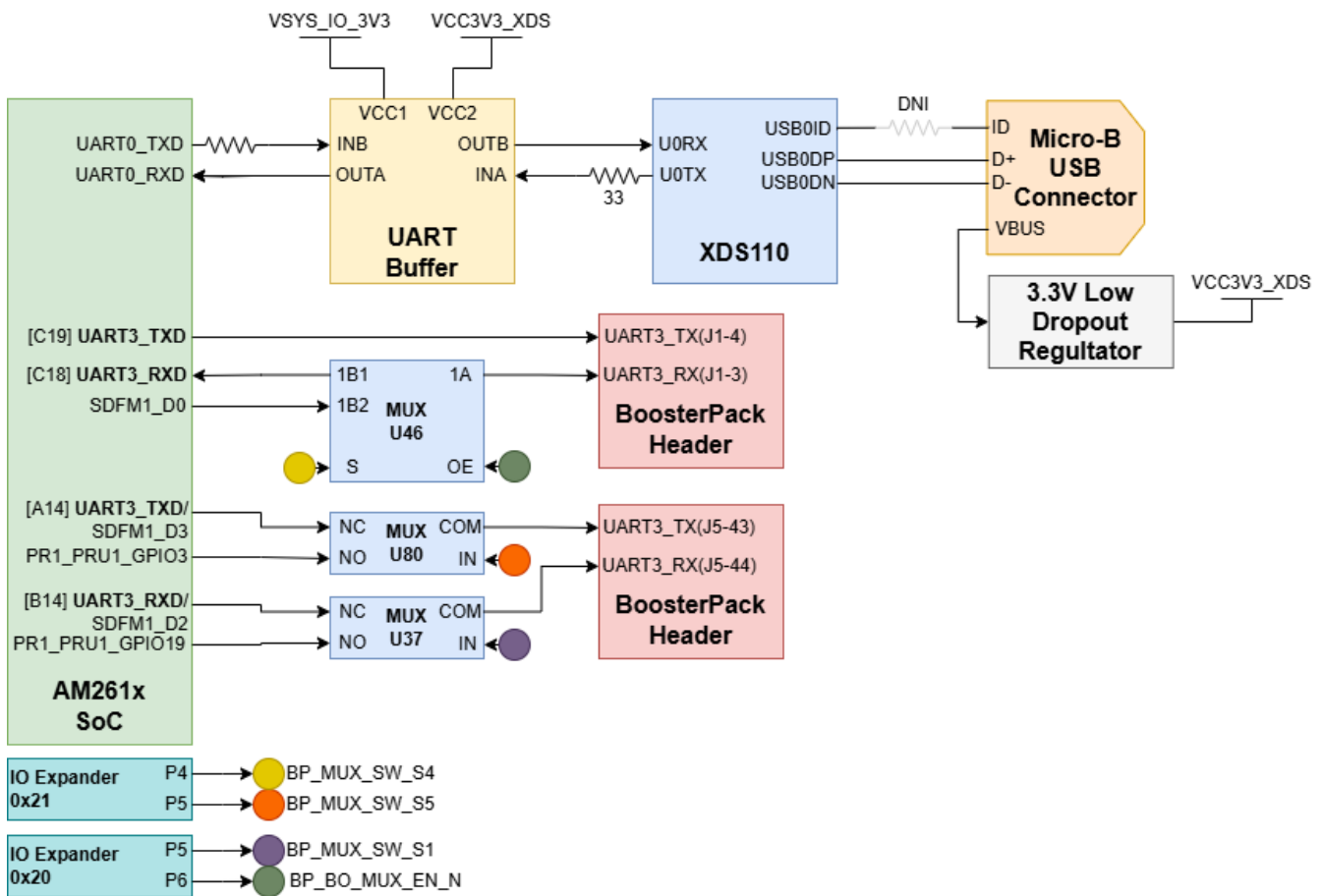
Figure 2-21. LP-AM261 UART Interface
