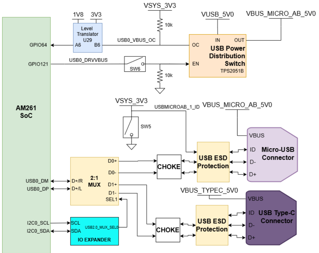
Figure 2-34. LP-AM261 USB Interface
