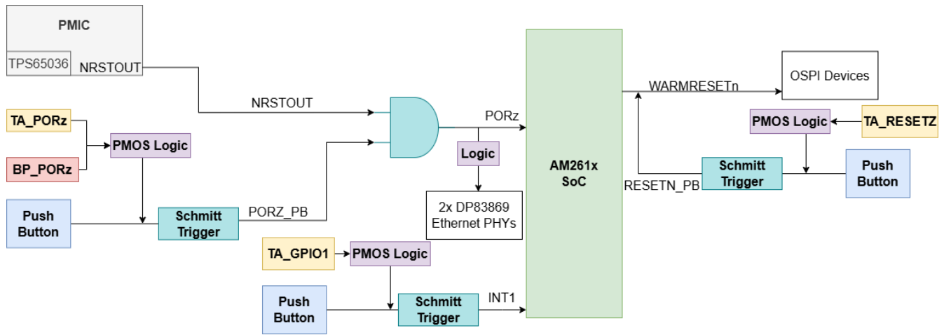
Figure 2-7. Reset Architecture
