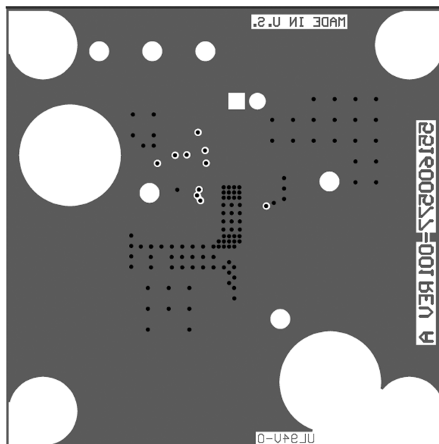
Figure 11. Bottom Layer
