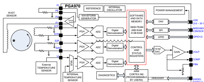
Figure 2. PGA970 Block Diagram
