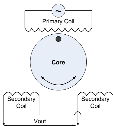
Figure 1. RVDT Mechanism
