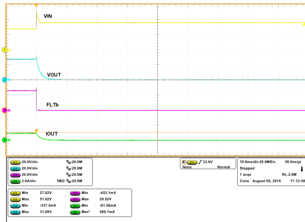
Figure 6. LM76202-Q1EVM Output Overvoltage Protection ( V_{IN} = 36\text{ V} , I_{LIM} = 2.23\text{ A} , R_{OUT} = 28\ \Omega , MODE = RTN )
