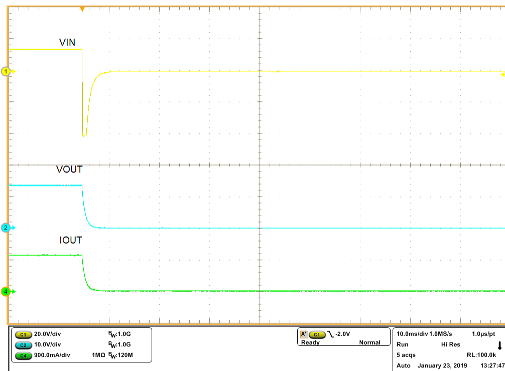
Figure 8. LM76202-Q1EVM Negative Input Voltage Transient Test (12-V battery voltage, transient voltage = -150 V , R_{LOAD} = 12 \Omega )
