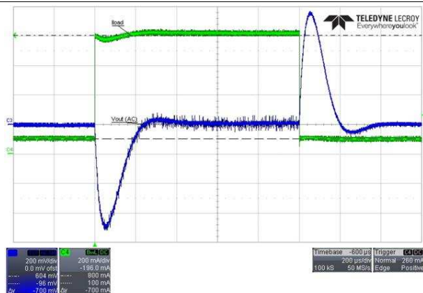
Figure 33. Load-Step Response V_{IN} = 14\text{ V} , V_{OUT} = 12\text{ V} (Buck Mode), 100 mA-800 mA-100 mA
