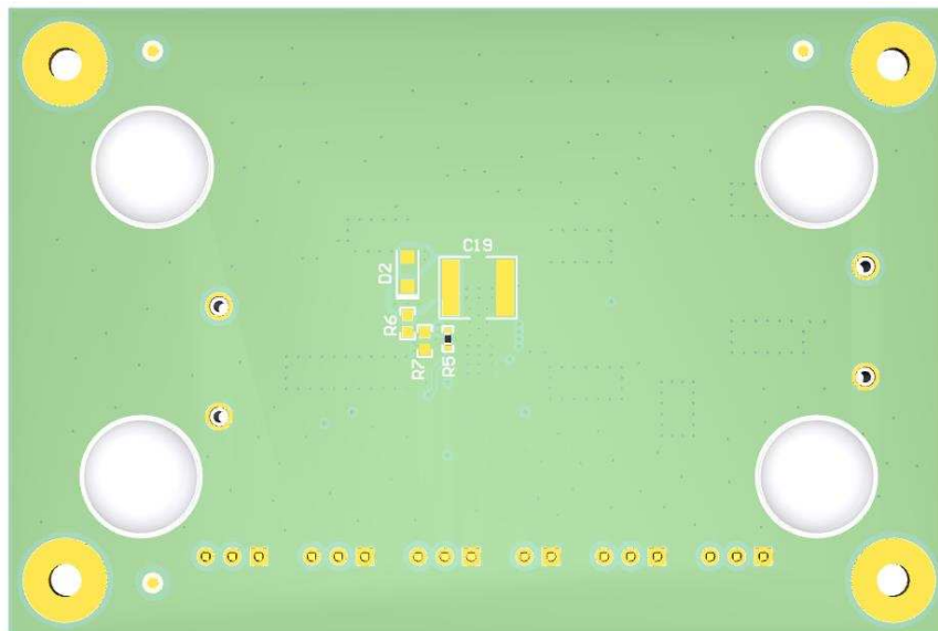
Figure 9. Component Placement—Bottom
