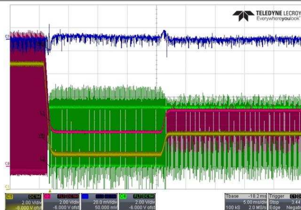
Figure 38. Cranking Pulse Response With 5-V Output, 200-mA Load, Zoom to 5 ms/div
