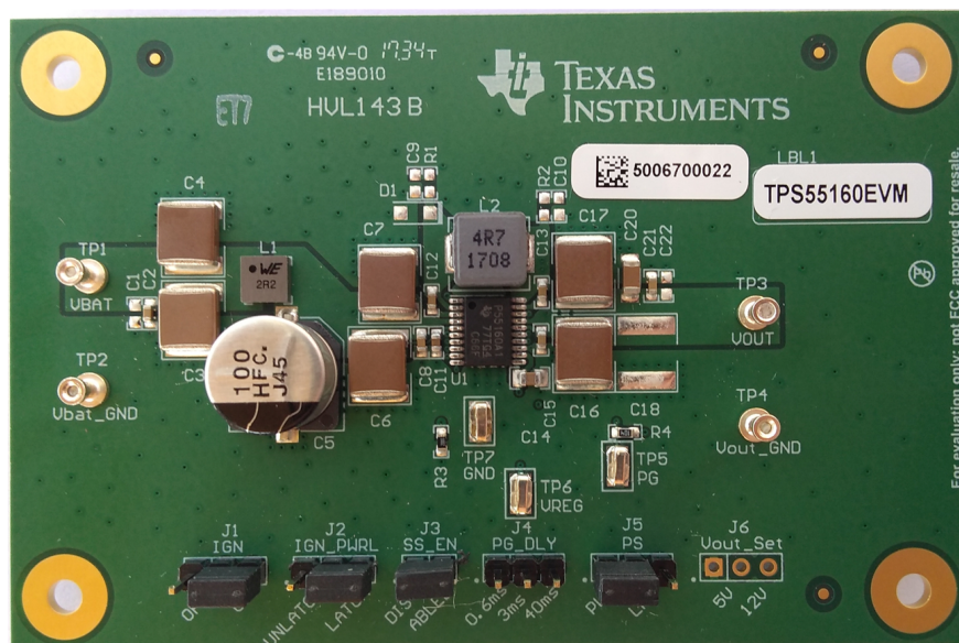
Figure 1. TPS55160Q1-EVM With Jumper Settings
