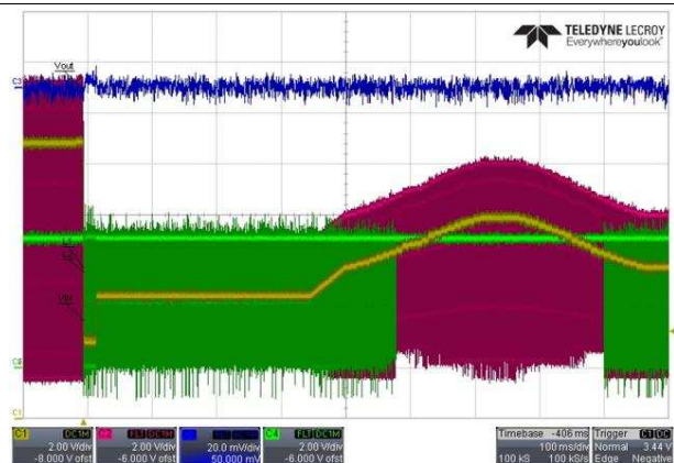
Figure 37. Cranking Pulse Response With 5-V Output, 200-mA Load, Zoom to 100 ms/div
