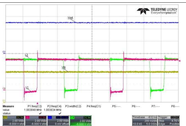
Figure 29. Switch-Nodes in Buck-Boost-Mode ( V_{IN} = 5 V, V_{OUT} = 5 V)
