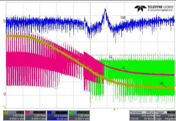
Figure 39. Cranking Pulse Response With 5-V Output, 200-mA load, Zoom to 200 µs/div
