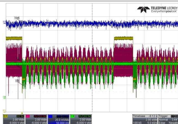
Figure 36. Cranking Pulse Response With 5-V Output, 200-mA Load, 2 s/div
