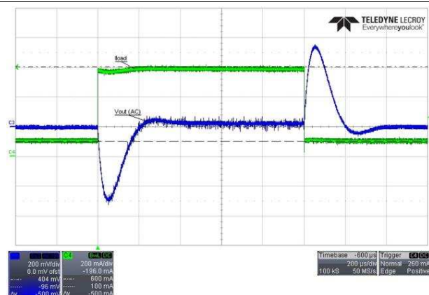
Figure 34. Load-Step Response V_{IN} = 12\text{ V} , V_{OUT} = 12\text{ V} (Buck-Boost Mode), 100 mA-600 mA-100 mA
