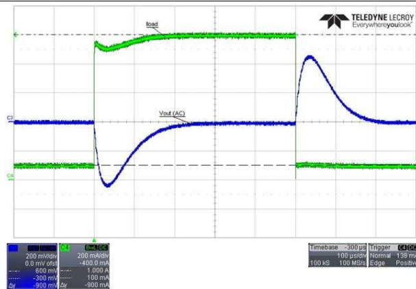
Figure 31. Load-Step Response V_{IN} = 12\text{ V} , V_{OUT} = 5\text{ V} (Buck Mode), 100 mA-1 A-100 mA
