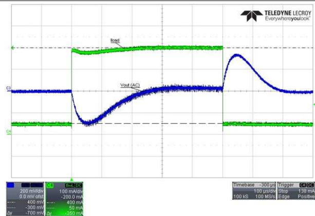
Figure 32. Load-Step Response V_{IN} = 2.5\text{ V} , V_{OUT} = 5\text{ V} (Boost Mode), 50 mA-400 mA-50 mA
