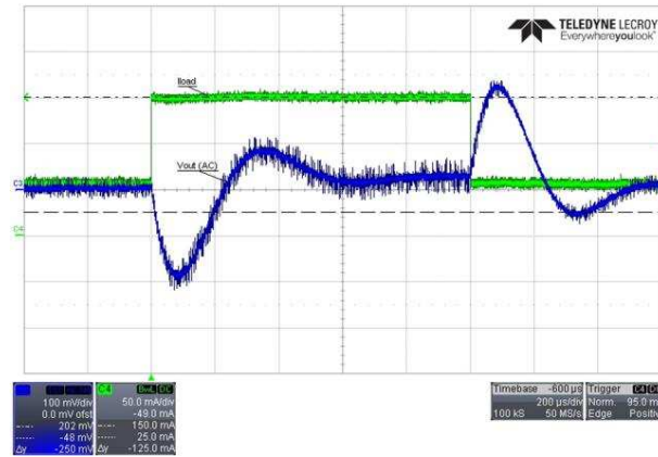
Figure 35. Load-step-response V_{IN} = 4\text{ V} , V_{OUT} = 12\text{ V} (Boost Mode), 50 mA-150 mA-50 mA
