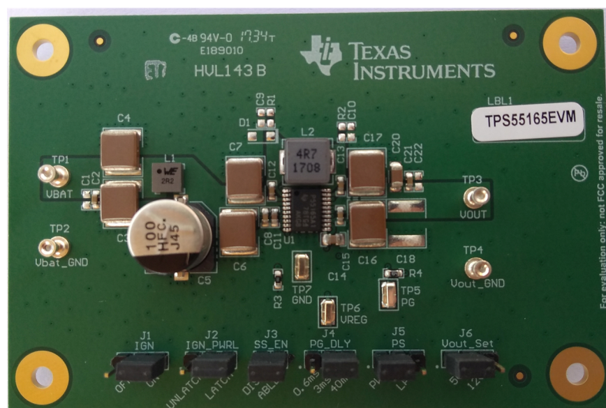
Figure 2. TPS55165Q1-EVM With Jumper Settings
