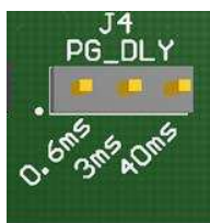
Figure 20. Power-Good Delay Selection Jumper Configuration Default: Jumper Not Installed, 3-ms Delay
