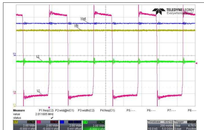
Figure 28. Switch-Nodes in Buck Mode ( V_{IN} = 12 V, V_{OUT} = 5 V)
