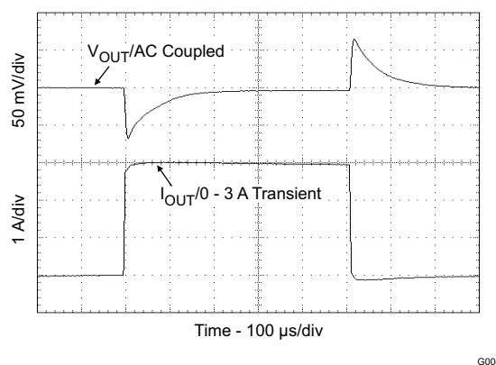
Figure 5. TPS54678EVM-155 Transient Response
