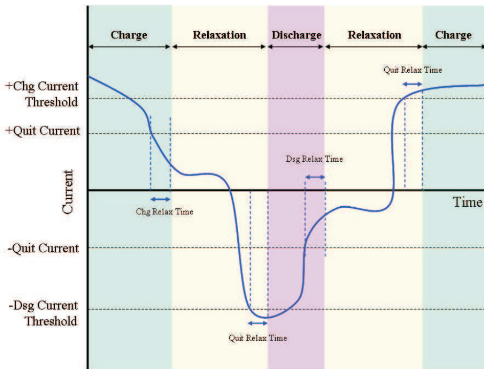
Figure 7-1. Example of Algorithm Operation Mode Changes with Varying DataRAM.Average Current()
