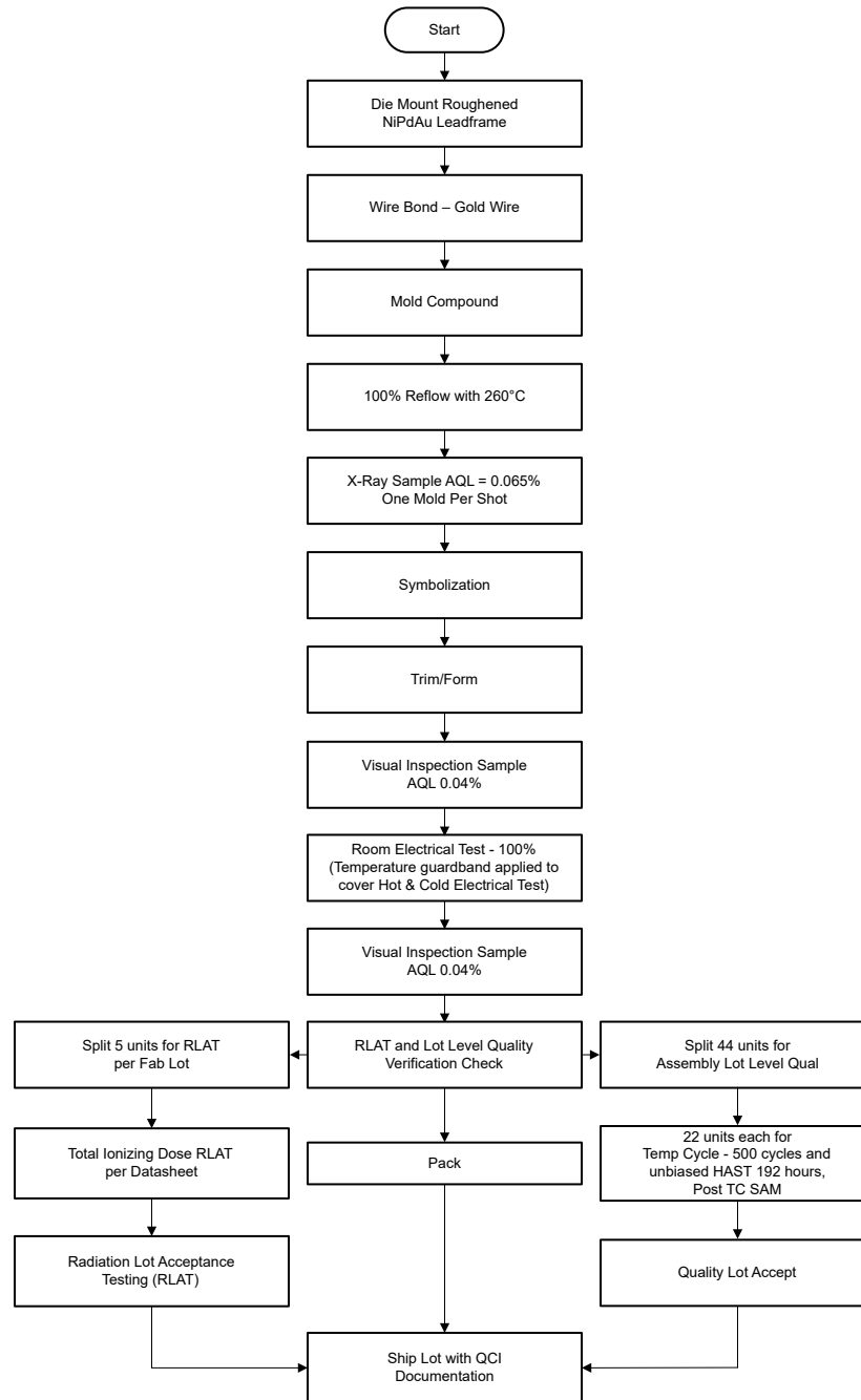
Figure 1-1. SN55LVRA4-SEP Space Enhanced Plastic Production Flow Chart
