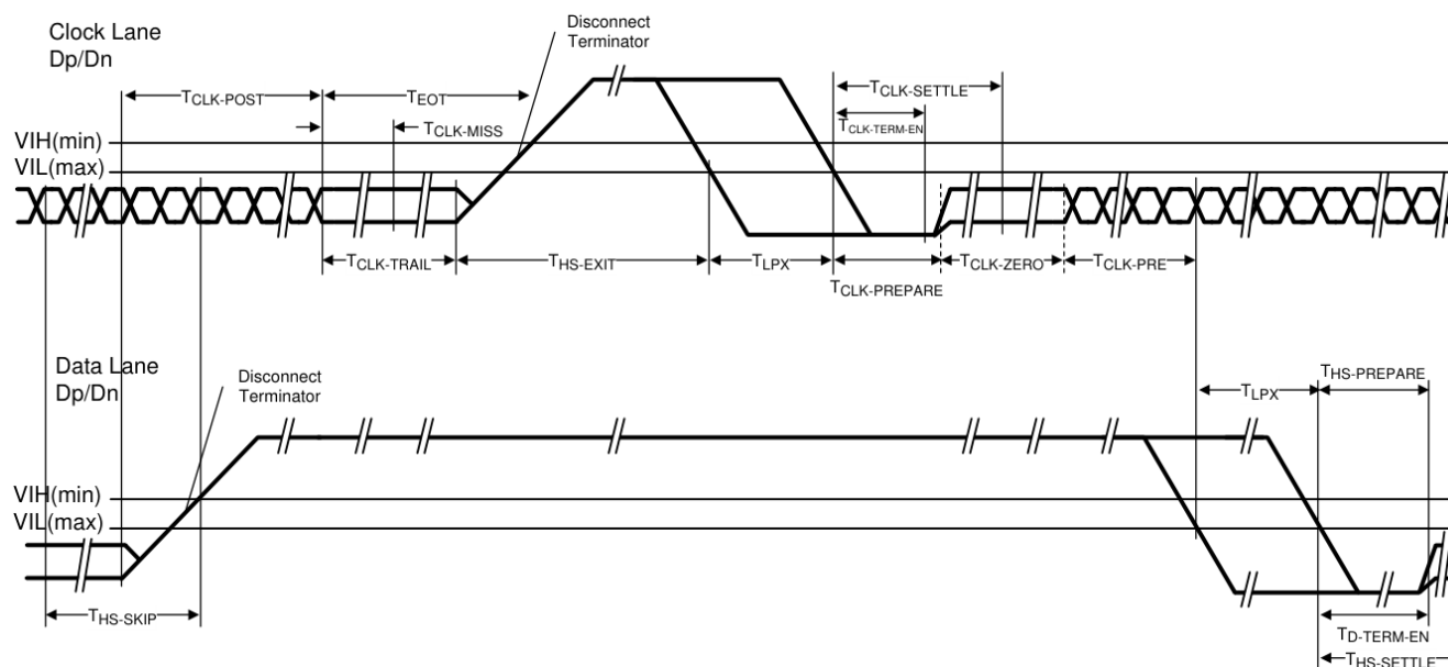
Figure 3-5. High Speed Data Transmission Burst
