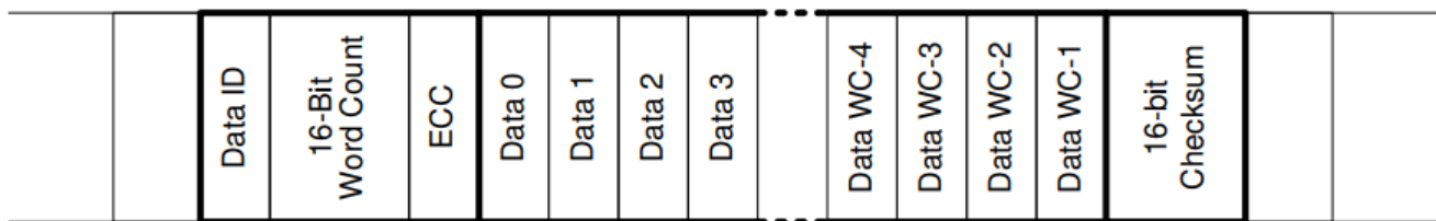
Figure 3-1. MIPI CSI-2 Long Packets
