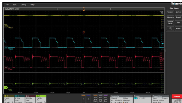
图 3-20. V_{in} = 230\text{Vac} , V_{out} = 15\text{V}
