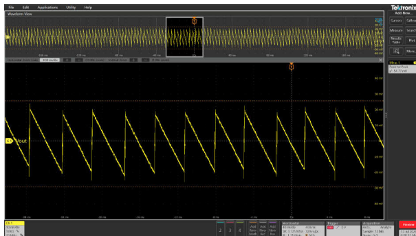
图 3-42. V_{OUT} = 20V 且无负载时的典型纹波电压 (55mVpp)
