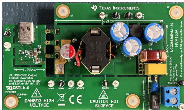
UCG28836EVM-150 (顶视图)
