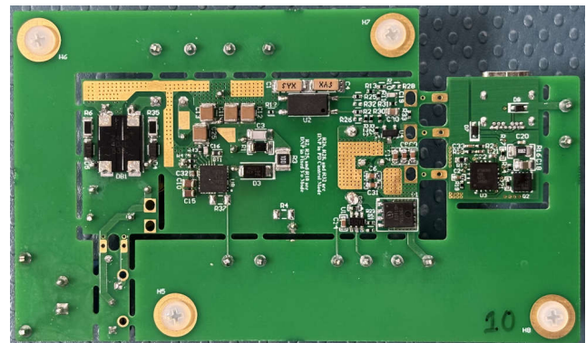
UCG28836EVM-150 (底视图)
