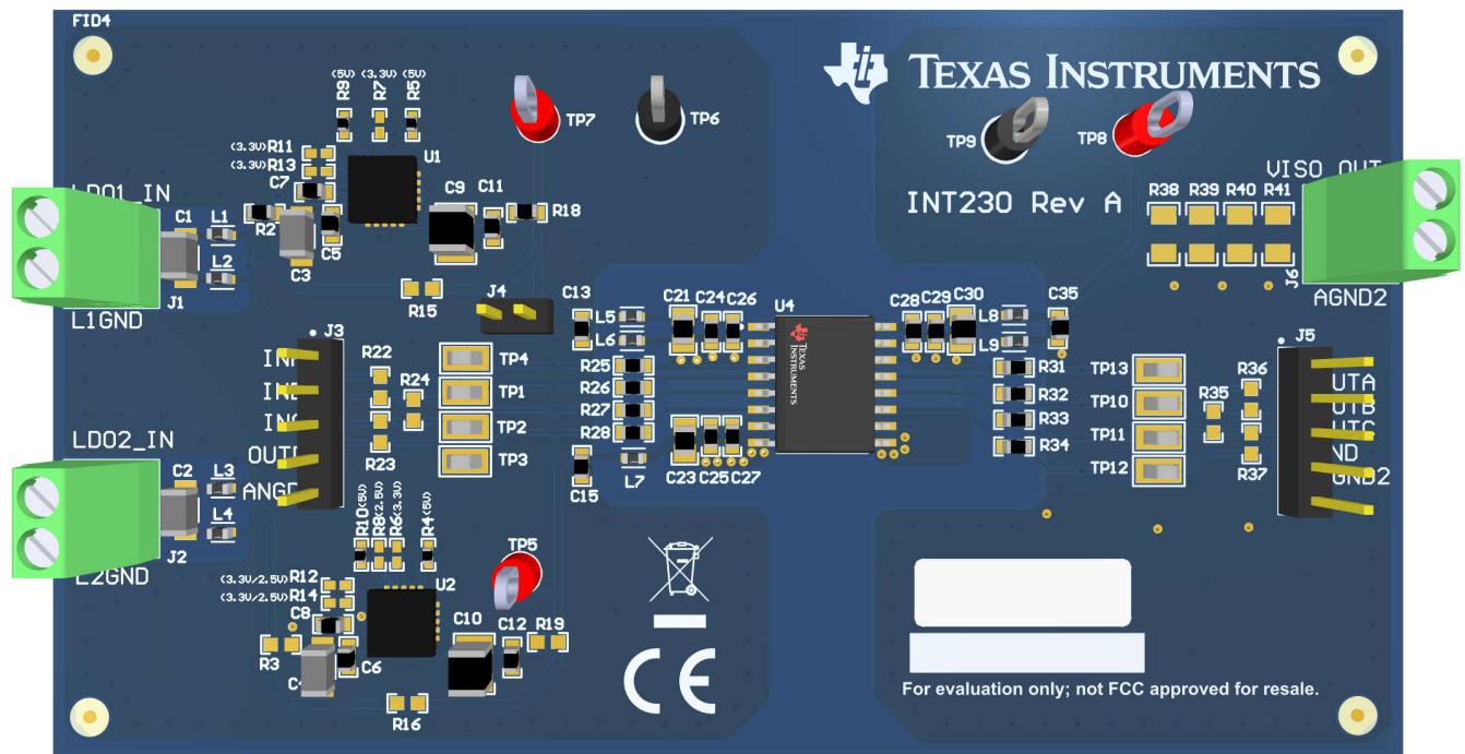
ISOW6441DWEEVM
