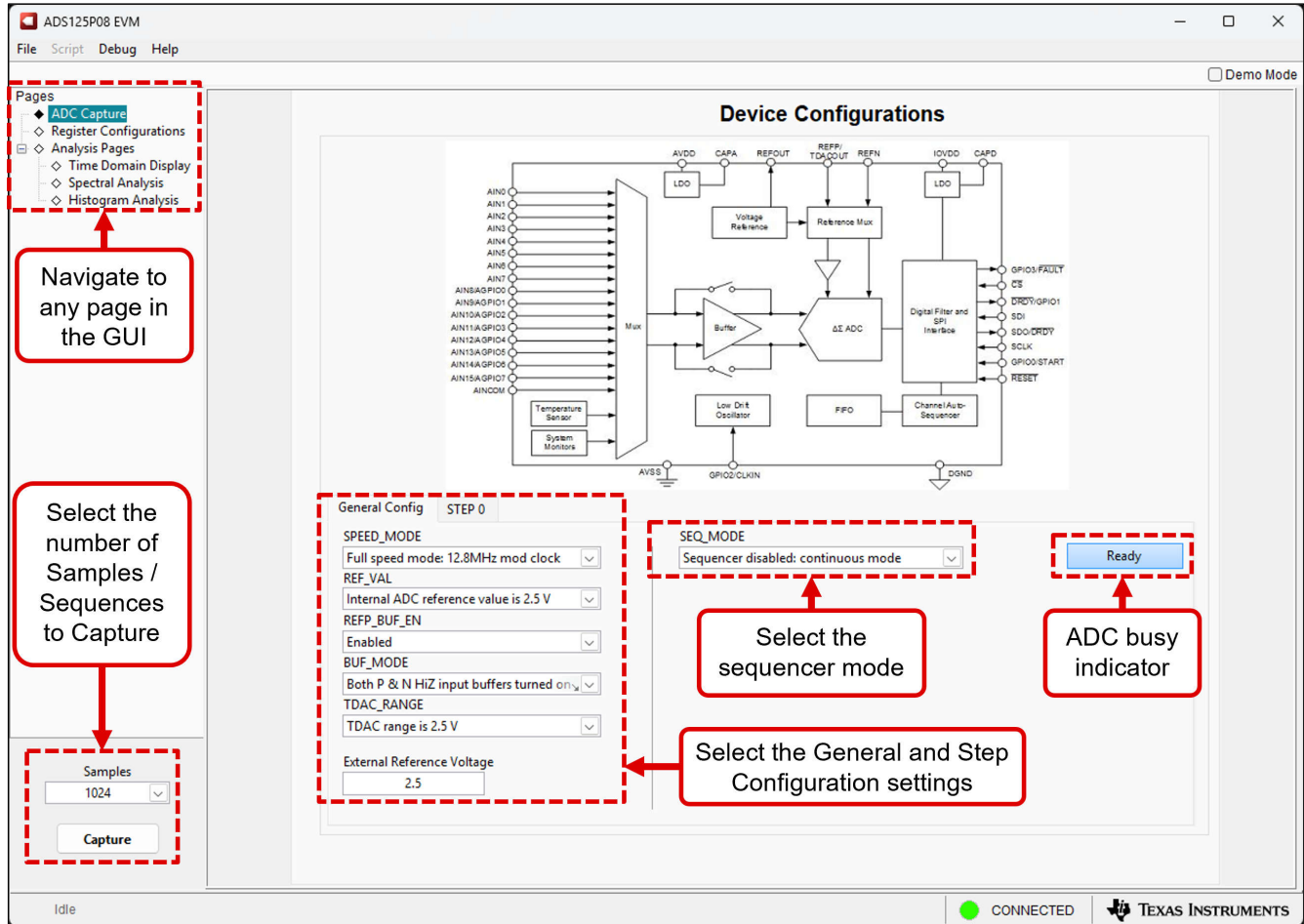
图 4-3. ADS125P08 EVM GUI ADC Capture 页面 — General Configuration
