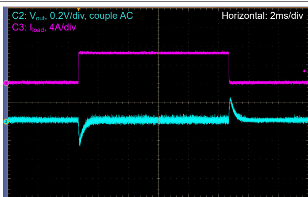
图 3-8. 负载瞬态, V_{in} = 14.4V , V_{out} = 24V , FPWM, I_{load} = 0A 至 6.25A , 1A/\mu s
