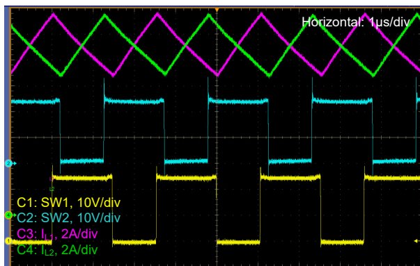
图 3-6. V_{in} = 14.4V , V_{out} = 24V , DEM, I_{load} = 15A
