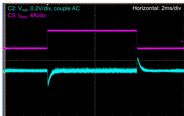
图 3-7. 负载瞬态, V_{in} = 14.4V , V_{out} = 24V , FPWM, I_{load} = 0A 至 6.25A , 1A/\mu s
