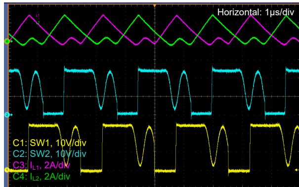
图 3-5. V_{in} = 14.4V , V_{out} = 24V , DEM, I_{load} = 1A
