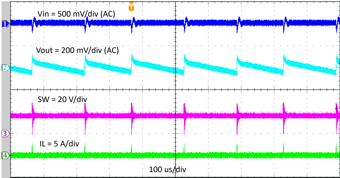
图 3-1. TPS56837HEVM 输出电压纹波 ( V_{IN} = 24V , I_{OUT} = 0.01A )
