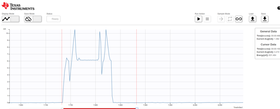
图 28. Sensor current consumption for reception of 150-Byte Data
