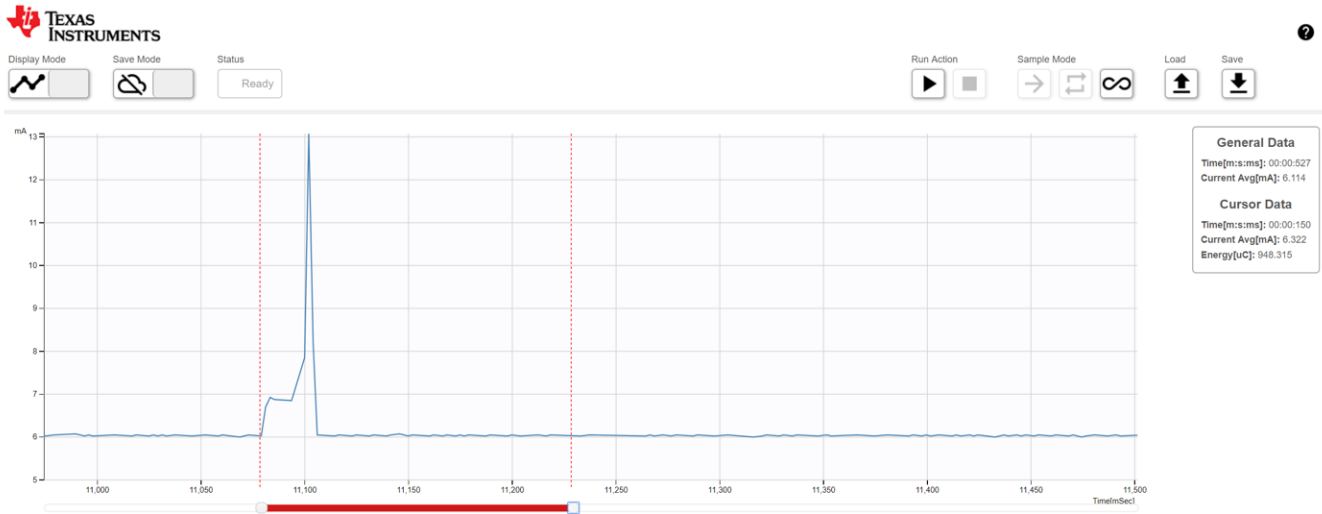
图 35. Collector Current Consumption for Receiving 70-Byte Data
