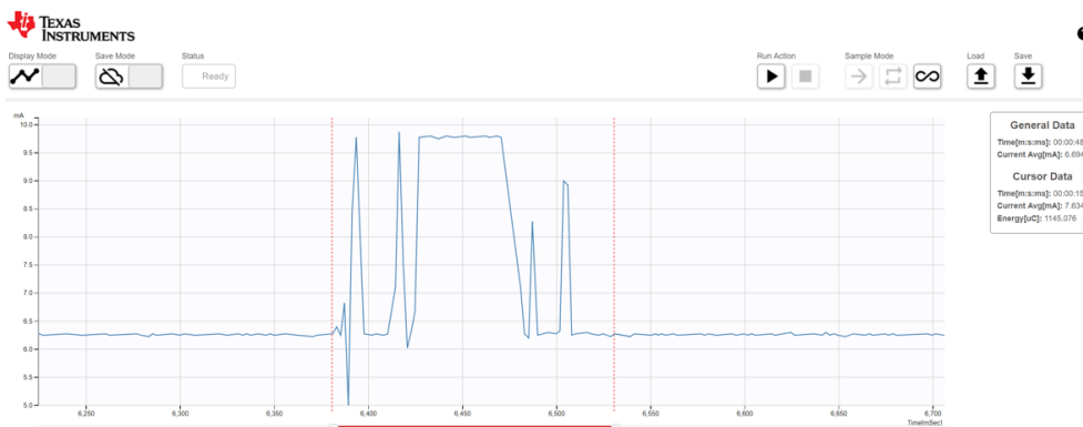
图 32. Collector Current Consumption for Transmission of 300-Byte Data
