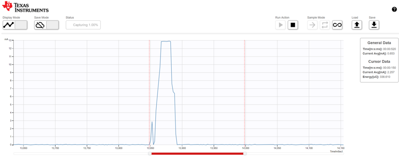
图 33. Sensor Current Consumption for Transmitting 70-Byte Data
