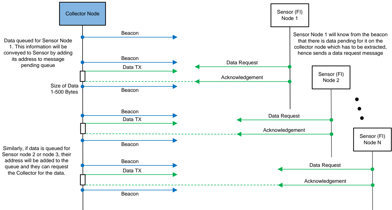
图 15. Data Exchange Between Sensor and Collector
