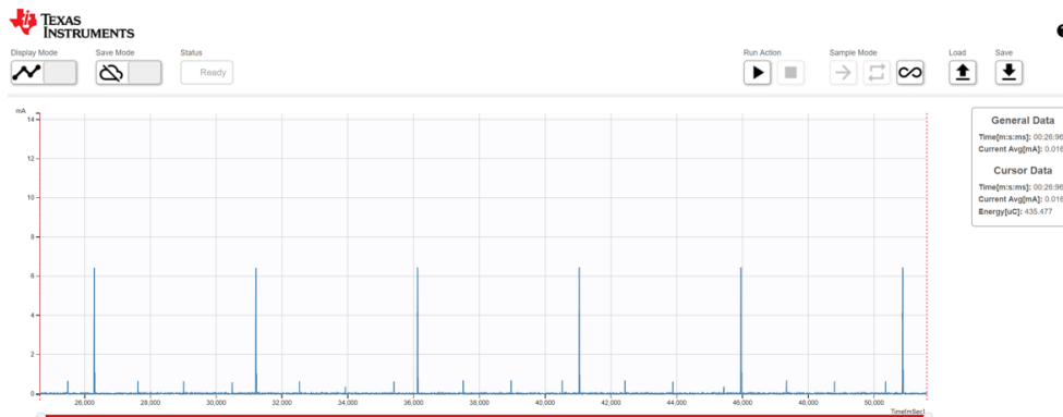
图 18. Sensor Current Consumption for a Beacon Interval of 4.92 s
