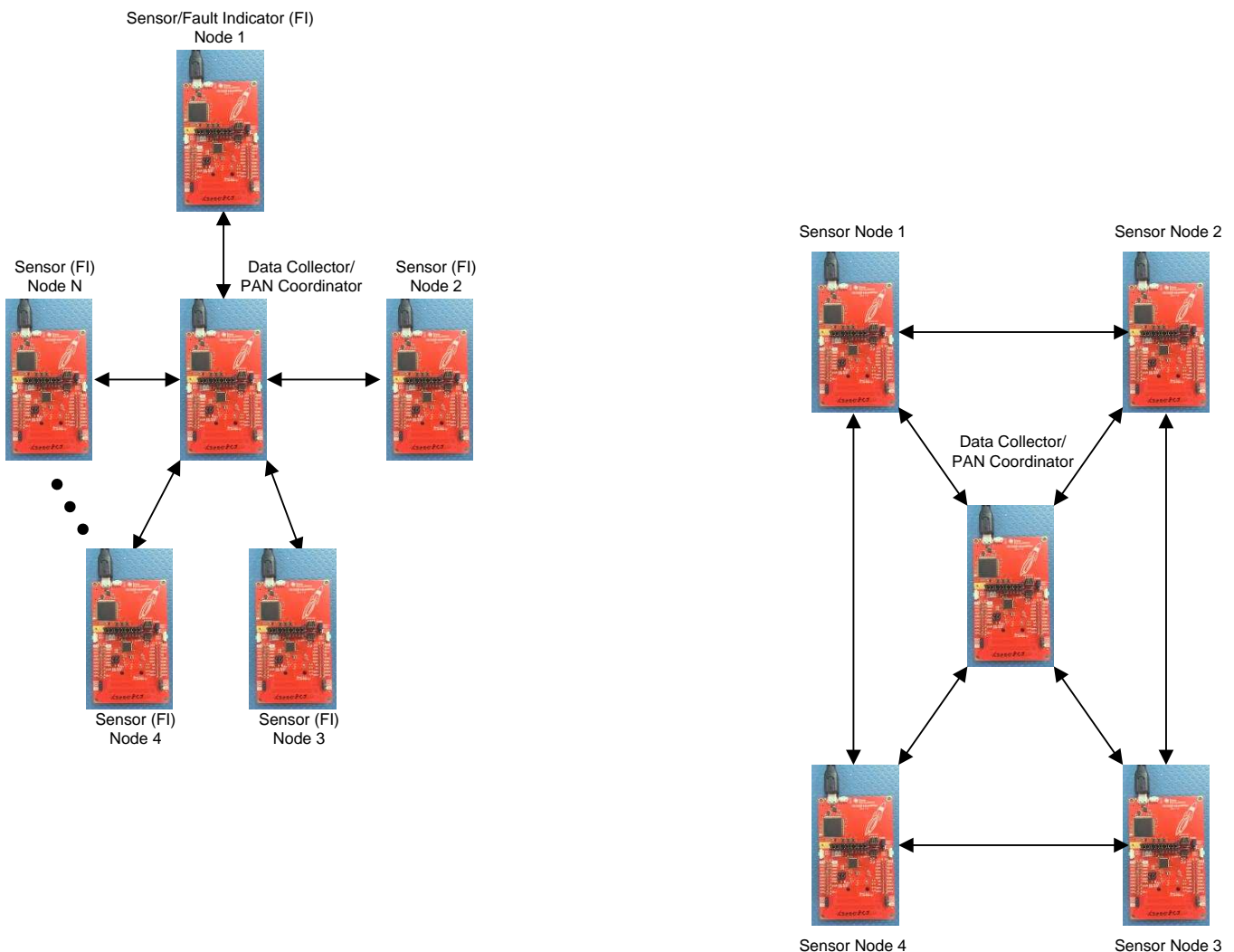
图 2. Star and Peer-to-Peer Topology Network
