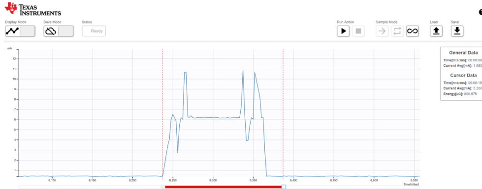
图 29. Sensor Current Consumption for Reception of 300-Byte Data
