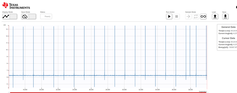
图 22. Collector Current Consumption for a Beacon Interval of 1.23 s
