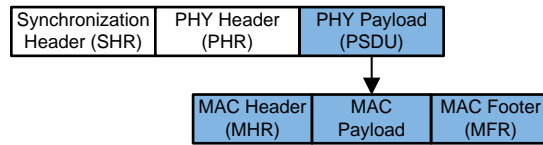
图 3. Schematic View of PDU
