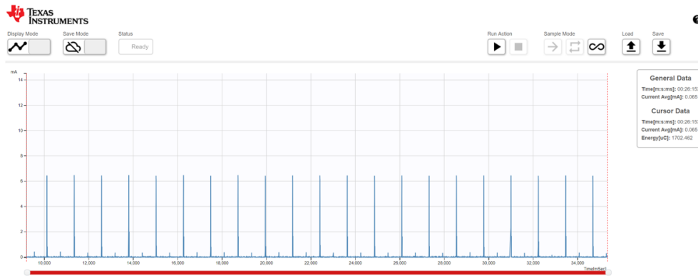
图 19. Sensor Current Consumption for a Beacon Interval of 1.23 s
