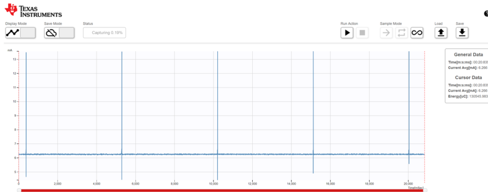
图 21. Collector Current Consumption for a Beacon Interval of 4.92 s
