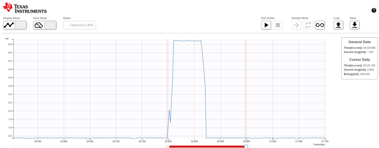
图 34. Sensor Current Consumption for Transmitting 300-Byte Data
