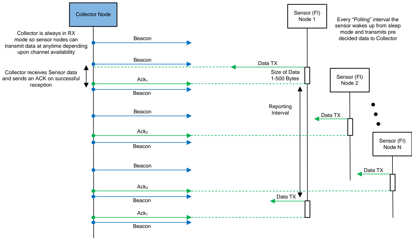
图 14. Status Report From Sensor (FPI) to Collector
