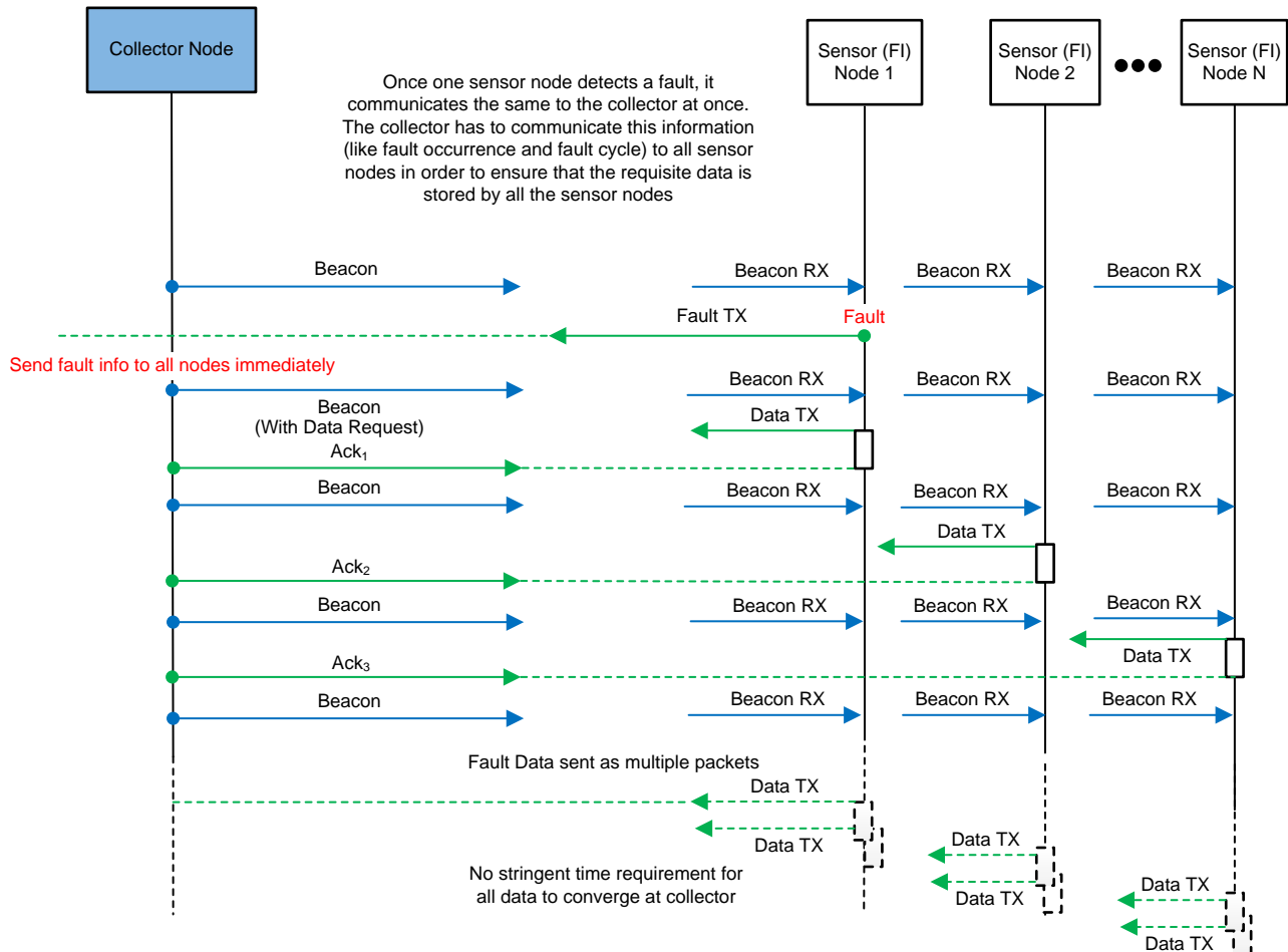
图 16. Fault Detection and Fault Information Broadcast
