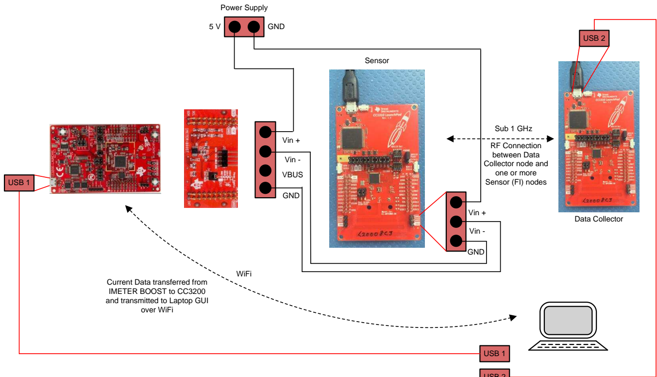
图 17. TIDA-00816 Test Setup for Current Measurement
