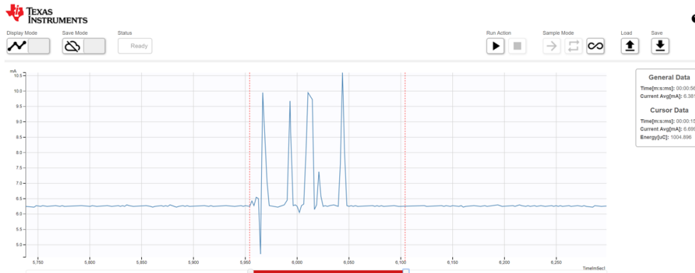
图 30. Collector Current Consumption for Transmission of 1-Byte Data
