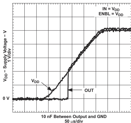
图 6-23. Output Behavior vs VDD (Noninverting)
