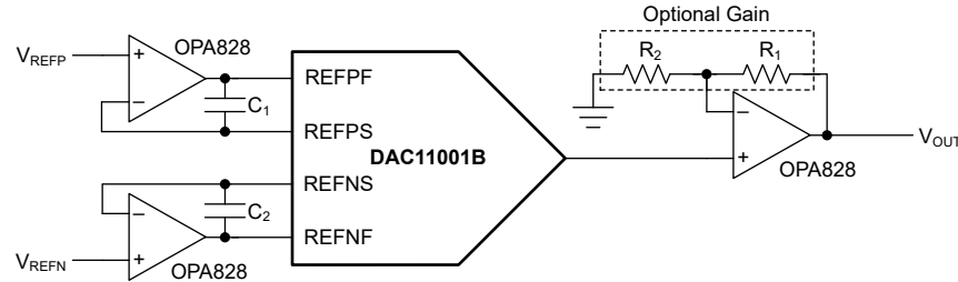
图 8-7. Arbitrary Waveform Generation
