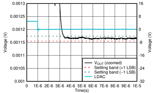
图 6-40. 100 Codes Settling Time, Falling Edge
