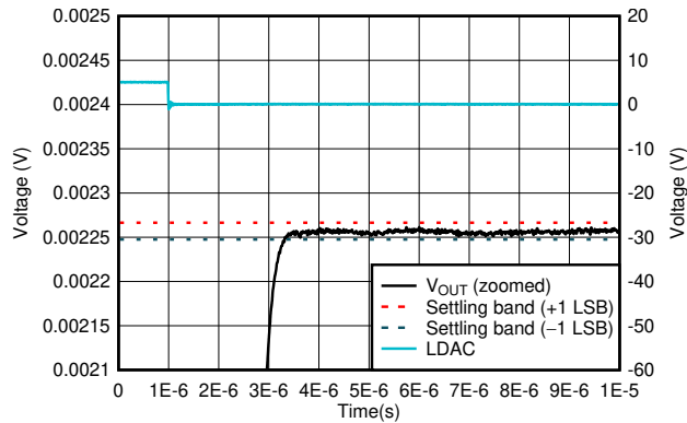
图 6-39. 100 Codes Settling Time, Rising Edge
