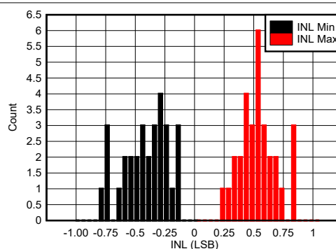
图 10-2. Typical INL Distribution After Reflow Soldering
