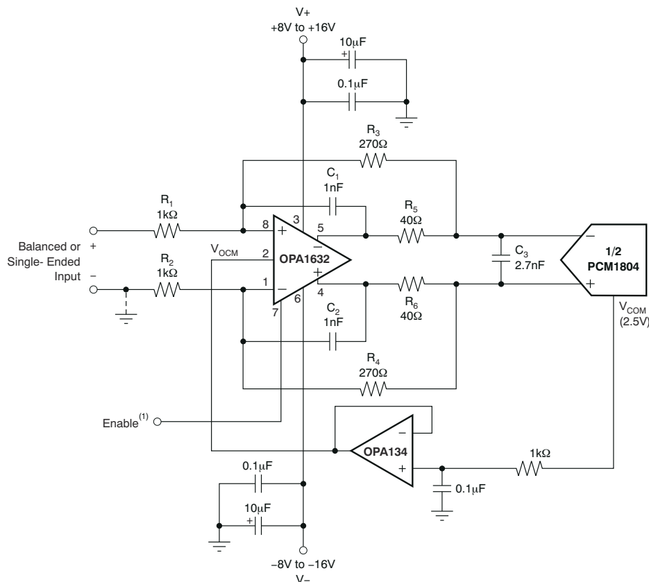
🔗 8-1. ADC Driver for Professional Audio
