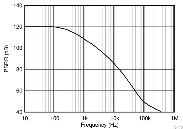
图 7-11. Power-Supply Rejection Ratio vs Frequency
