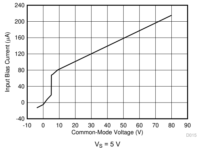
图 7-18. Input Bias Current vs Common-Mode Voltage
