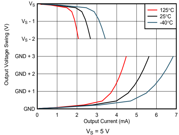
图 7-14. Output Voltage Swing vs Output Current
