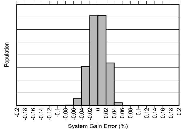
图 7-8. Gain Error Production Distribution (INA254A3)
