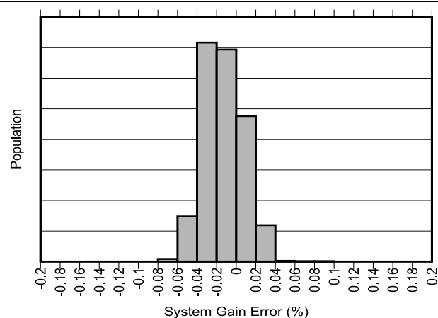
图 7-6. Gain Error Production Distribution (INA254A1)
