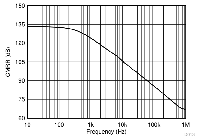
图 7-12. Common-Mode Rejection Ratio vs Frequency
