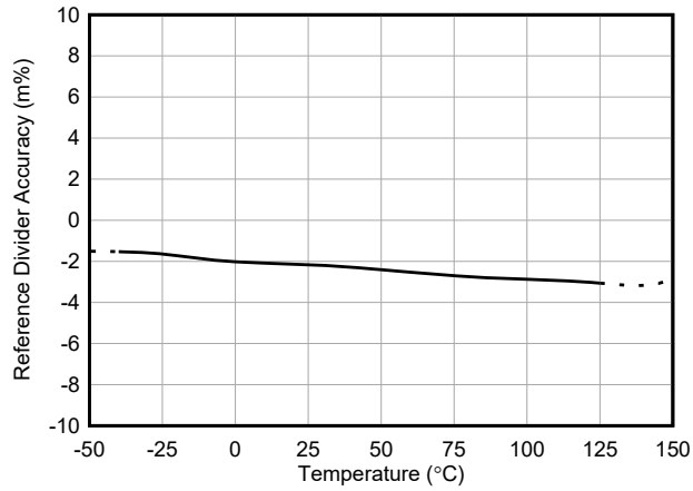
图 7-13. Reference Divider Accuracy vs Temperature
