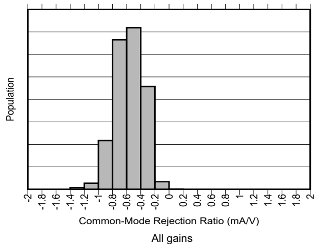
图 7-3. Common-Mode Rejection Production Distribution
