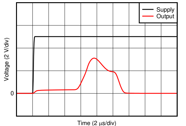
图 7-27. Amplifier Step Response
