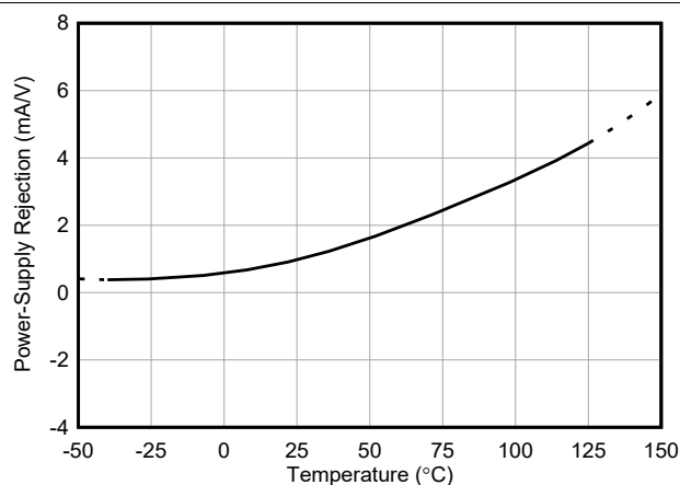
图 7-5. Power-Supply Rejection Ratio vs Temperature
