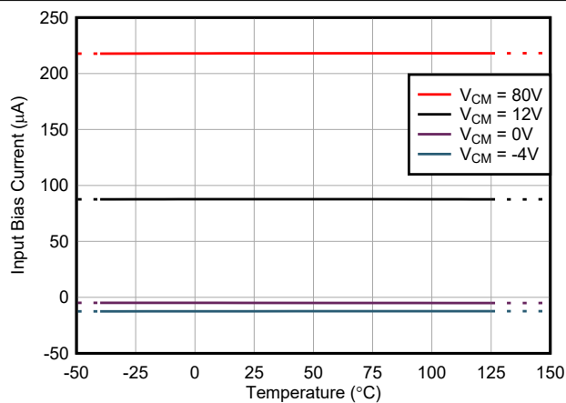
图 7-20. Input Bias Current vs Temperature
