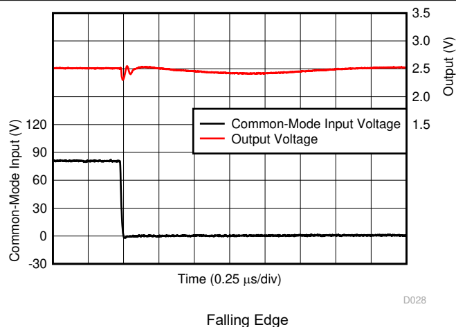
图 7-31. Common-Mode Voltage Transient Response
