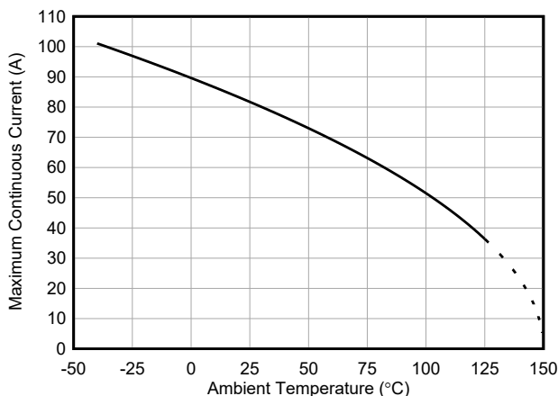
图 8-1. Maximum Continuous Current vs Ambient Temperature
