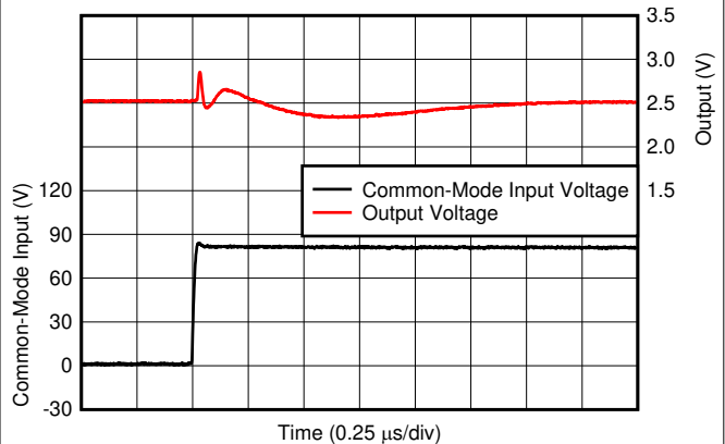
图 7-28. Common-Mode Transient Response
