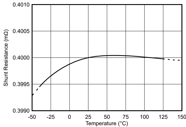
图 8-3. Sensing Resistor vs Temperature
