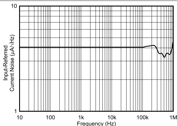
图 7-23. INA254A1 Input-Referred Current Noise vs Frequency
