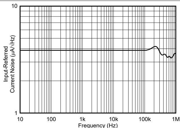
图 7-24. INA254A2 Input-Referred Current Noise vs Frequency
