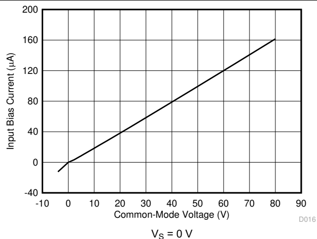
图 7-19. Input Bias Current vs Common-Mode Voltage
