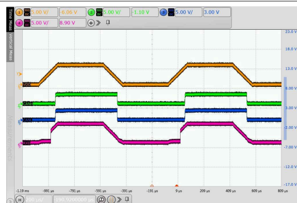
图 8-13. Glitch Free Power Up on VDD
