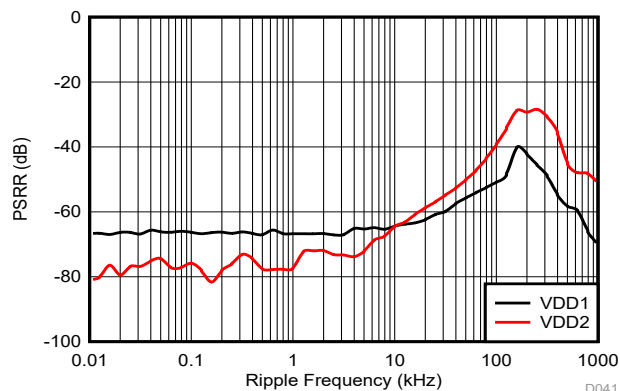
图 6-31. Power-Supply Rejection Ratio vs Ripple Frequency
