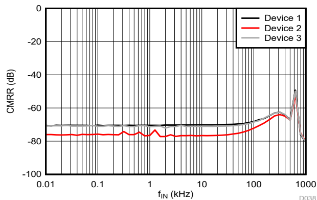
图 6-29. Common-Mode Rejection Ratio vs Input Frequency
