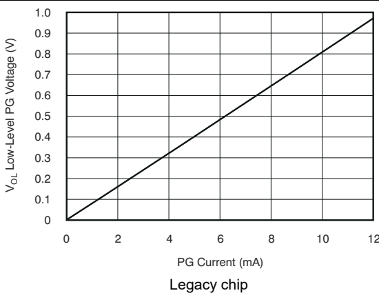
图 5-29. Low-Level PG Voltage vs Current
