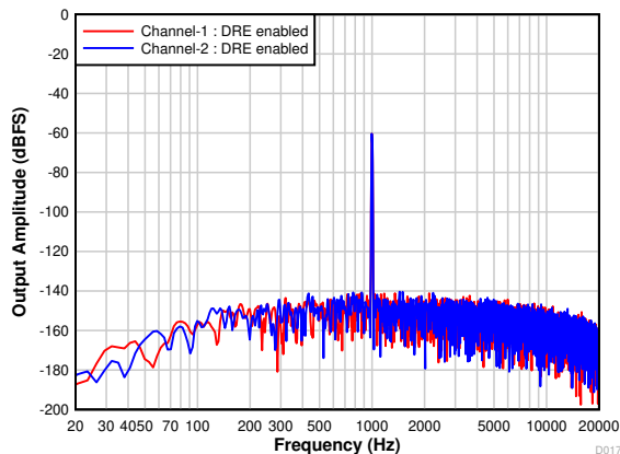
图 7-20. FFT With a -60-dBr Input With DRE Enabled
