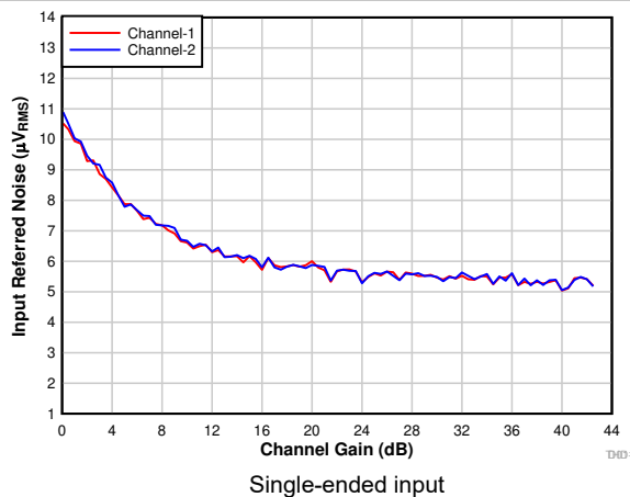
图 7-14. Input-Referred Noise vs Channel Gain
