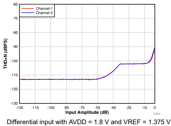
图 7-8. THD+N vs Input Amplitude With DRE Enabled
