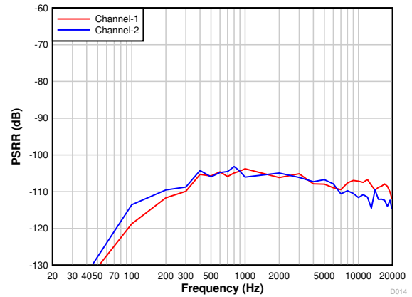
图 7-17. Power-Supply Rejection Ratio vs Ripple Frequency With 100-mV pp Amplitude
