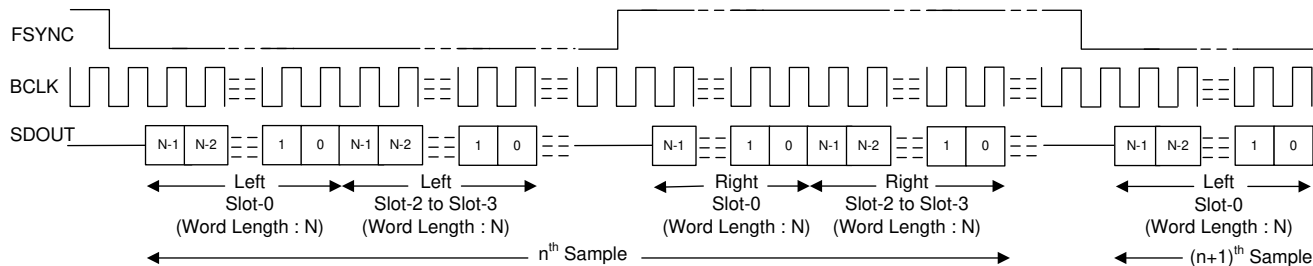
图 8-5. I 2 S Mode Standard Protocol Timing (TX_OFFSET = 0)
