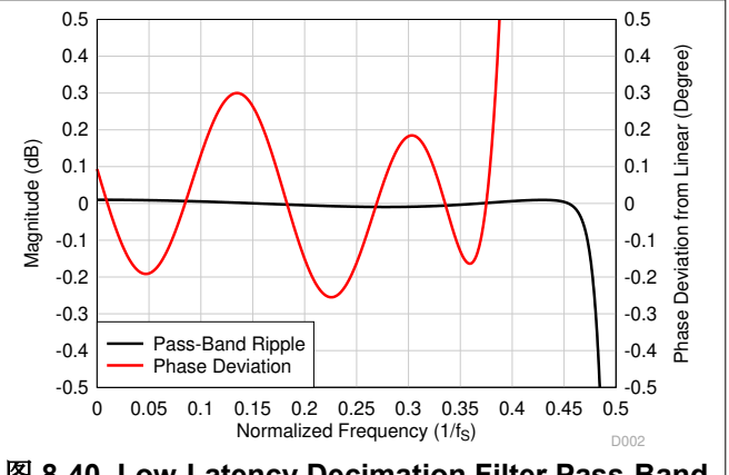
图 8-40. Low-Latency Decimation Filter Pass-Band Ripple and Phase Deviation
