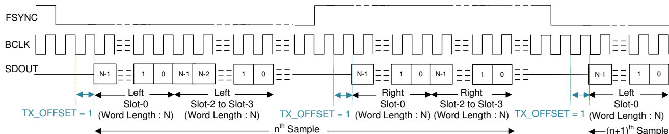
图 8-6. I 2 S Protocol Timing (TX_OFFSET = 1)
