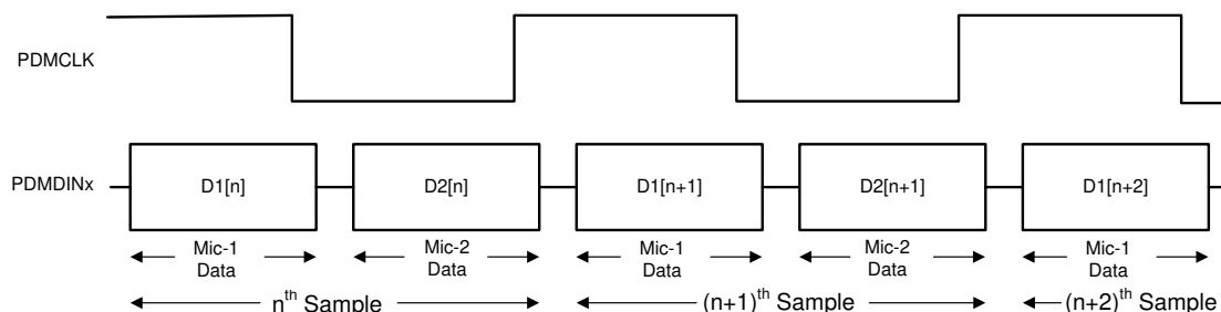
图 8-65. Digital PDM Microphone Protocol Timing Diagram
