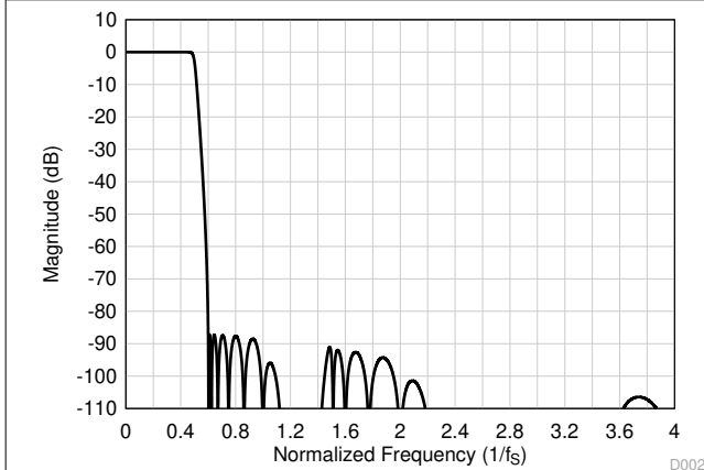
图 8-39. Low-Latency Decimation Filter Magnitude Response
