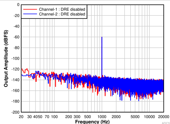
图 9-4. FFT With a - 60-dBr Input With DRE Disabled
