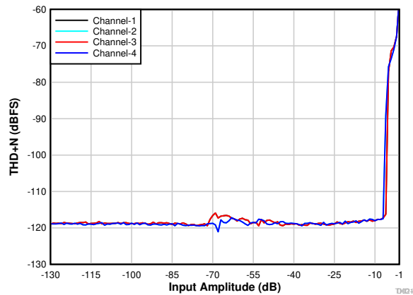
图 7-24. PDM Input THD+N vs Input Amplitude
