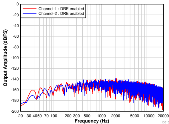
图 7-18. FFT With Idle Input With DRE Enabled
