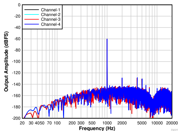
图 7-26. PDM Input FFT With a -60-dBr Input
