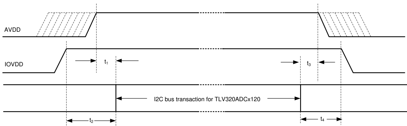
图 10-1. Power-Supply Sequencing Requirement Timing Diagram
