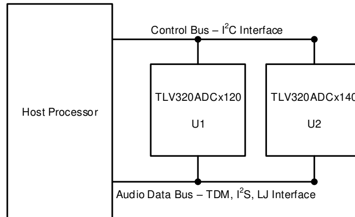
图 8-13. Multiple Devices With Shared Control and Audio Data Buses
