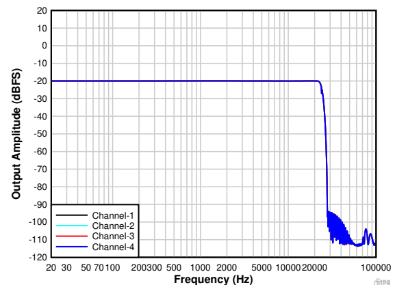
图 7-27. PDM Input Frequency Response With a -20-dBr Input
