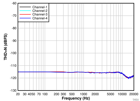
图 7-25. PDM Input THD+N vs Input Frequency With a -20-dBr Input
