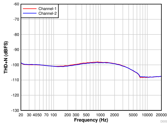
图 7-10. THD+N vs Input Frequency With a -60-dBr Input
