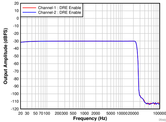
图 7-16. Frequency Response With a -30-dBr Input
