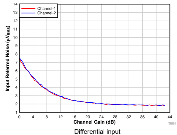
图 7-13. Input-Referred Noise vs Channel Gain
