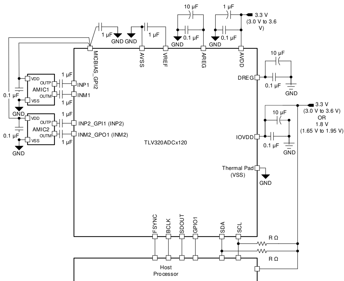
图 9-1. Two-Channel Analog Microphone Recording Diagram
