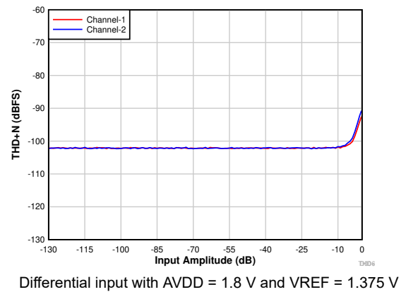
图 7-9. THD+N vs Input Amplitude With DRE Disabled
