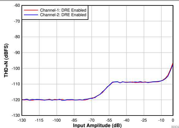
图 9-3. THD+N vs Input Amplitude With DRE Enabled
