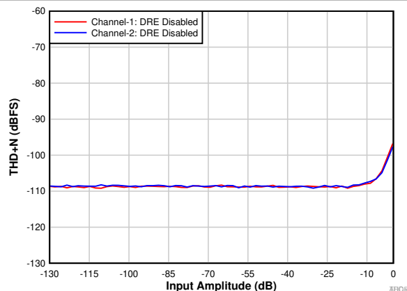
图 9-5. THD+N vs Input Amplitude With DRE Disabled
