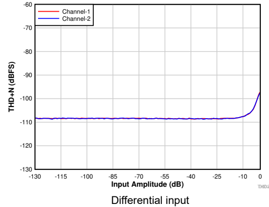
图 7-5. THD+N vs Input Amplitude With DRE Disabled
