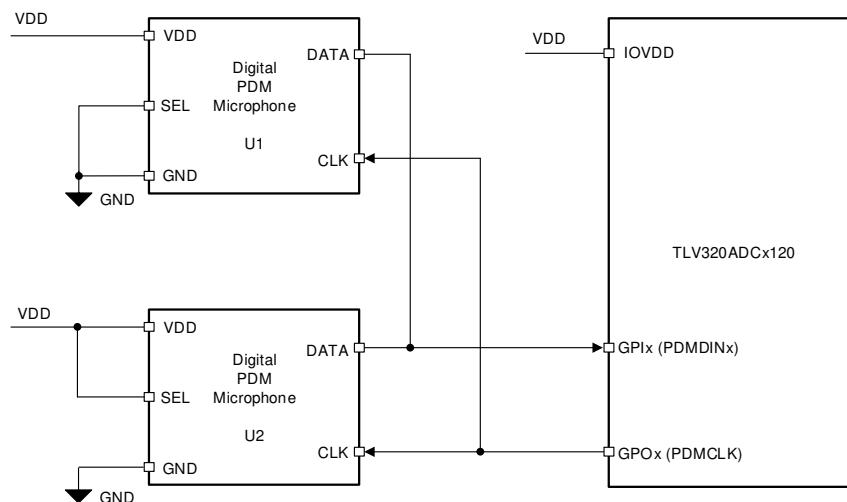
图 8-64. Digital PDM Microphones Connection Diagram for the TLV320ADC5120
