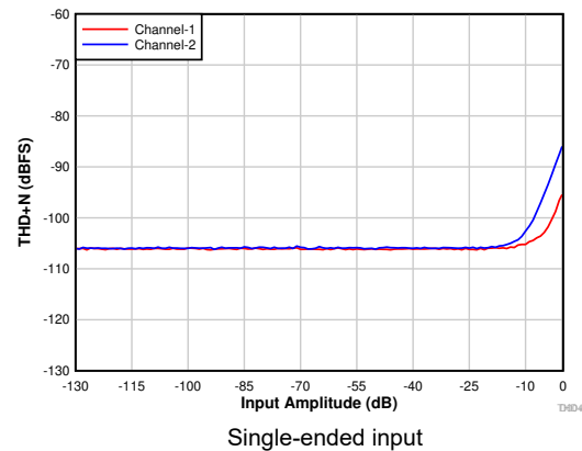
图 7-7. THD+N vs Input Amplitude With DRE Disabled
