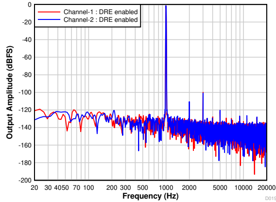
图 7-22. FFT With a -1-dBr Input With DRE Enabled
