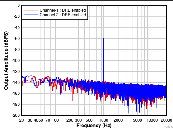
图 9-2. FFT With a - 60-dBr Input With DRE Enabled
