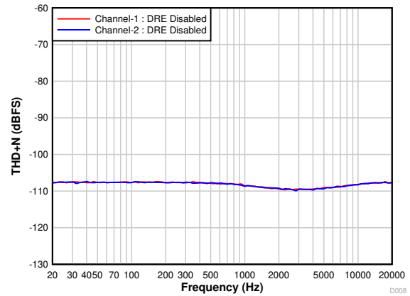
图 7-11. THD+N vs Input Frequency With a -60-dBr Input
