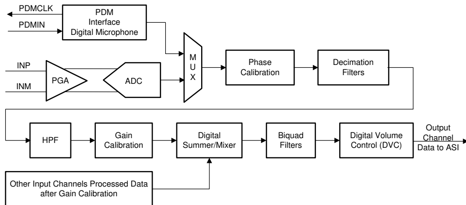
图 8-16. Signal-Chain Processing Flowchart
