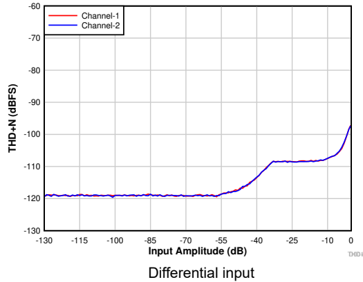
图 7-4. THD+N vs Input Amplitude With DRE Enabled
