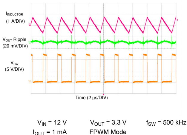
图 8-18. TPS7H4010-SEP Switching Waveform and V_{OUT} Ripple
