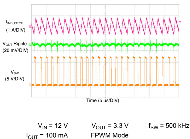
图 8-20. TPS7H4010-SEP Switching Waveform and V_{OUT} Ripple
