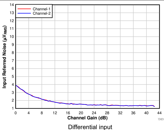
图 7-13. Input-Referred Noise vs Channel Gain
