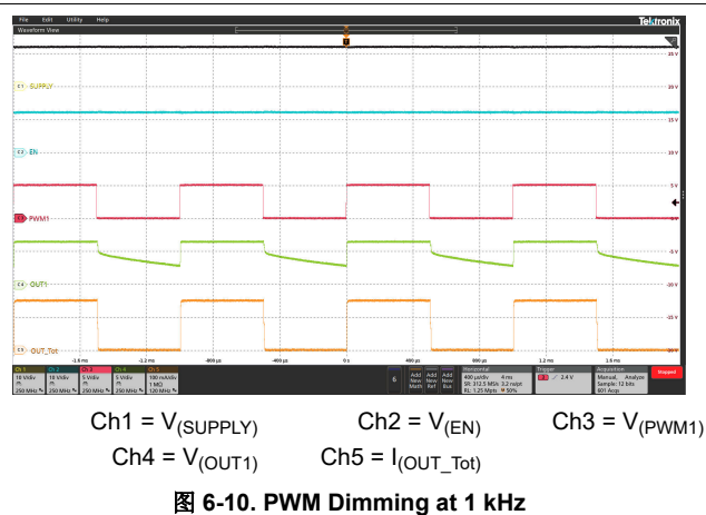
图 6-10. PWM Dimming at 1 kHz
