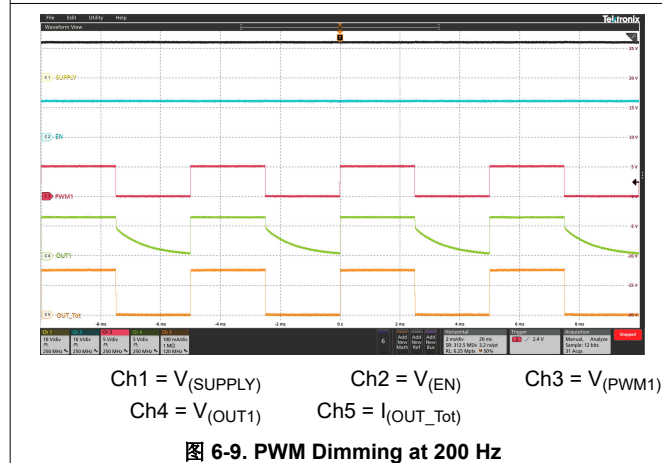
图 6-9. PWM Dimming at 200 Hz
