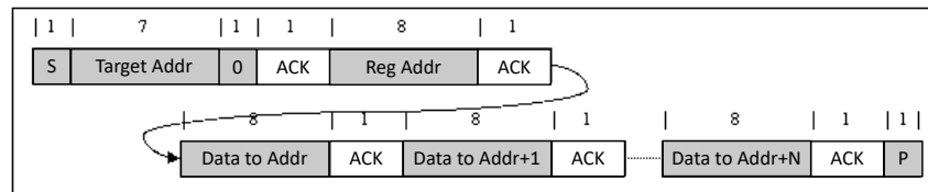
图 9-22. Multi-Write
