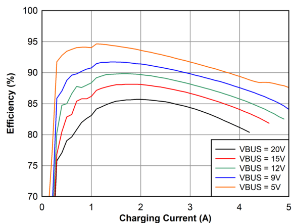
图 8-2. 1s Battery Charge Efficiency, 1.5 MHz
