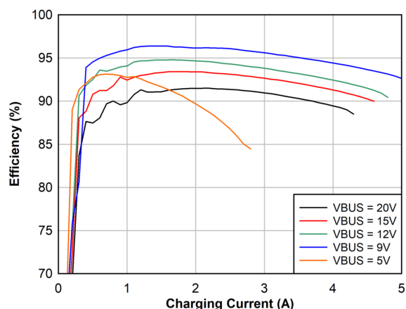
图 8-4. 2s Battery Charge Efficiency, 1.5 MHz
