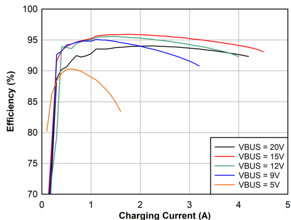
图 8-6. 3s Battery Charge Efficiency, 1.5 MHz
